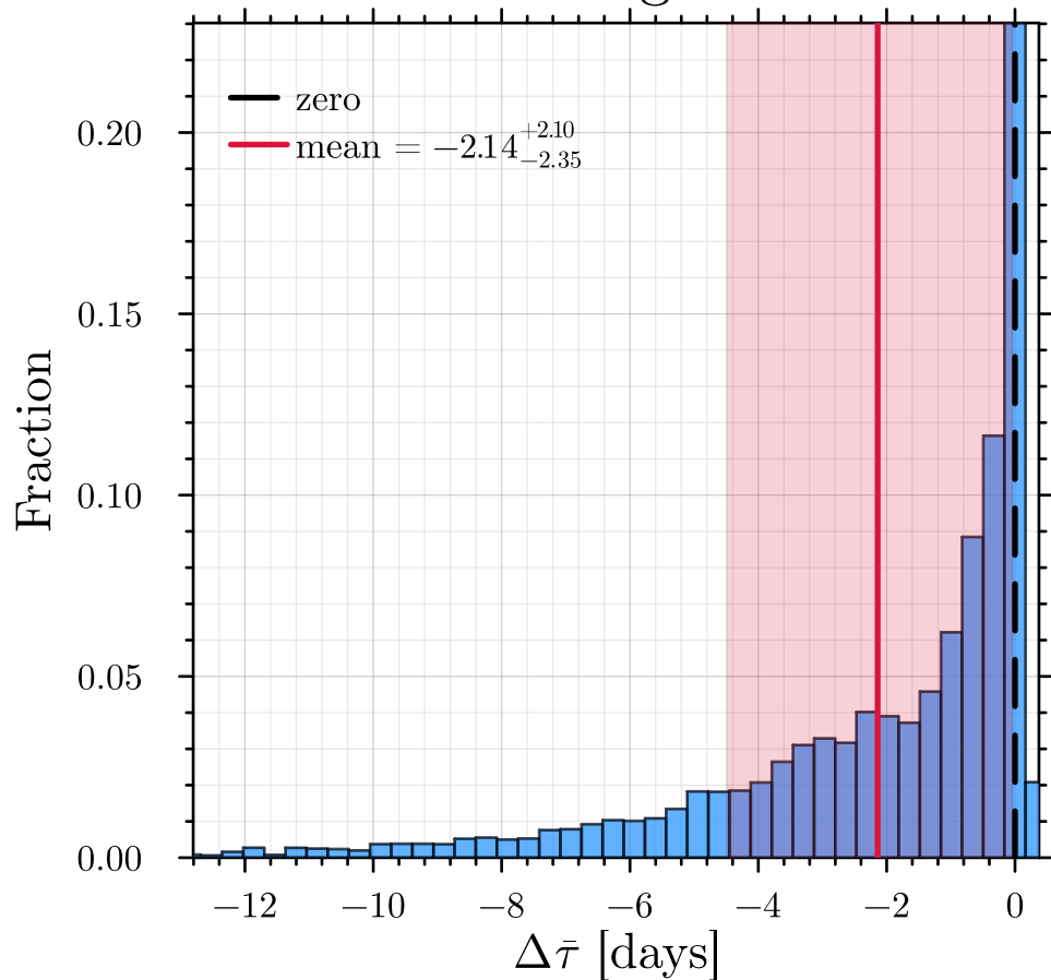
Centroid lag bias \Delta\bar{\tau}
