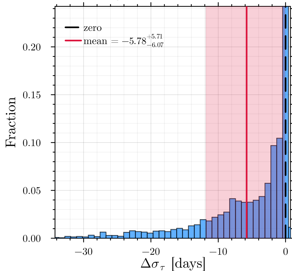
Lag extent bias \Delta\sigma_\tau
