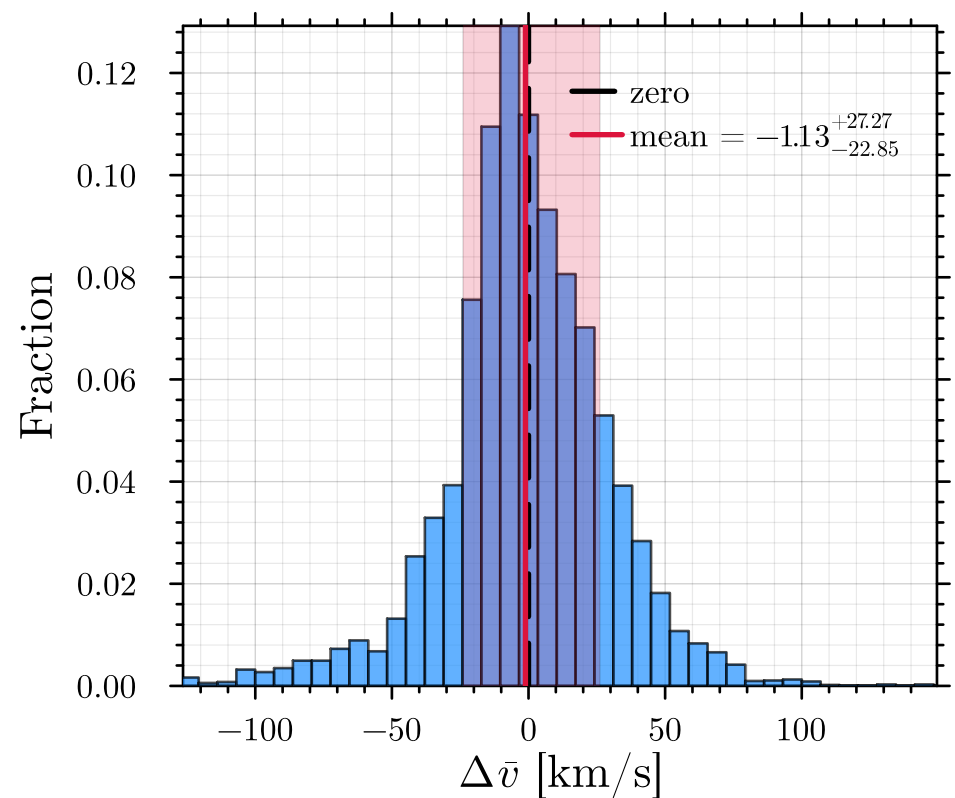
Centroid velocity bias \Delta\bar{v}
