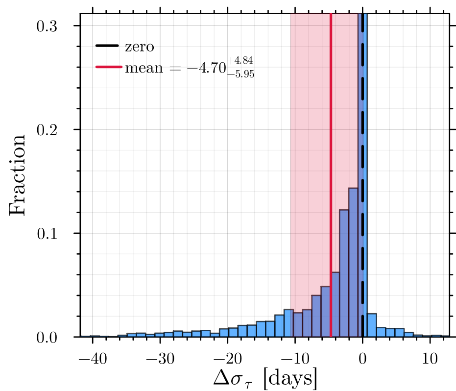
Lag extent bias \Delta\sigma_\tau
