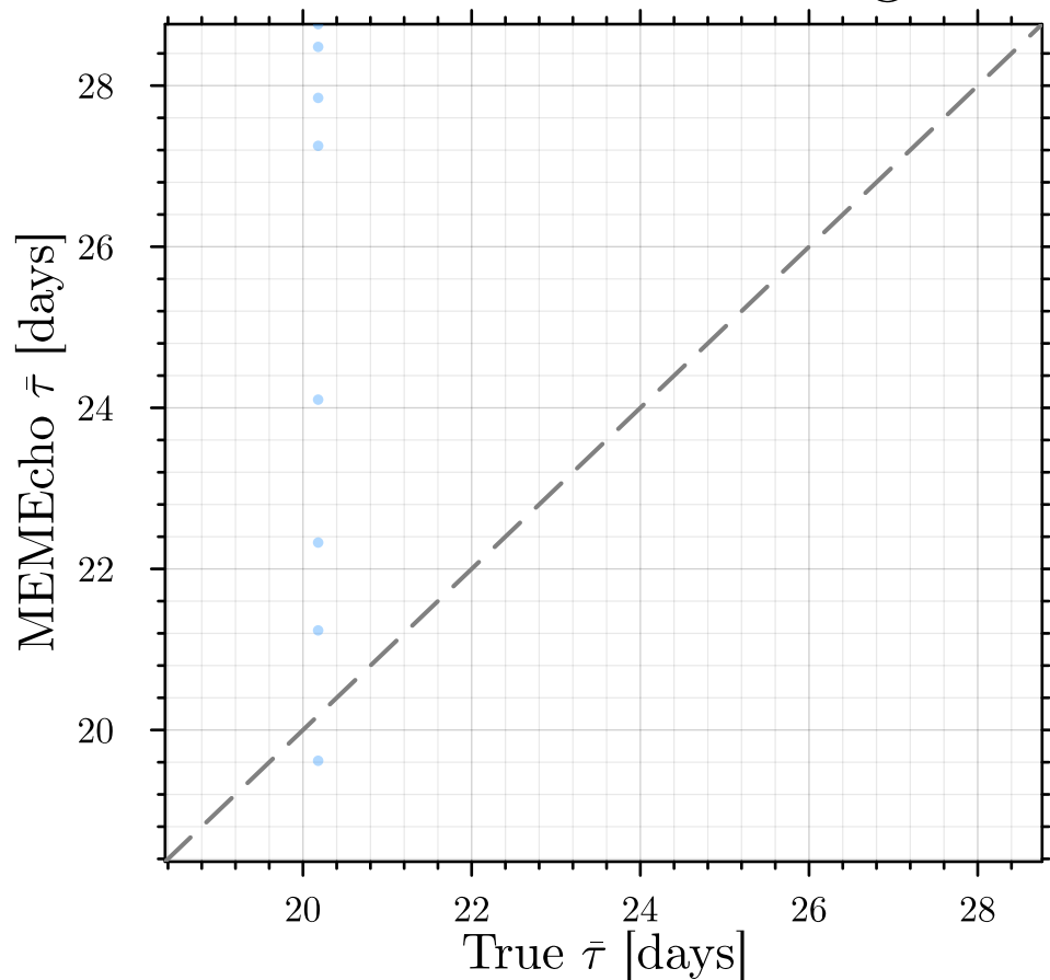
MEMEcho centroid lag \bar{\tau}
