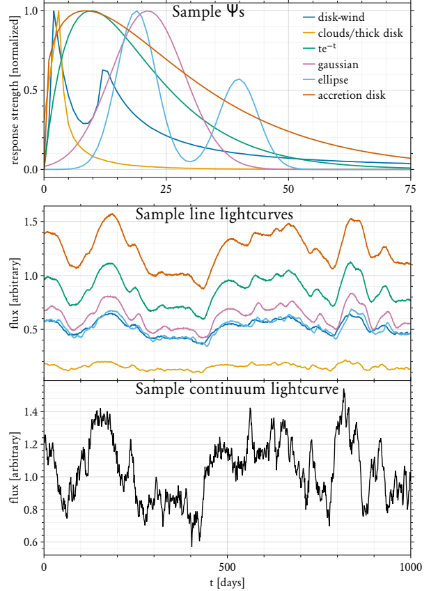
Figure 2. Top: Sample 1D transfer functions for each “basis” function used in training the model. Middle: Sample lightcurves resulting from the convolution of the corresponding transfer function from the top panel with the continuum. Bottom: The DRW continuum lightcurve convolved with the top panel to generate the middle panel.
