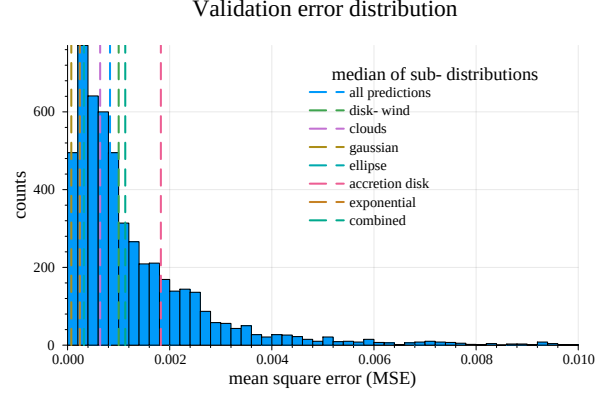
Figure 5. The distribution of errors for the sample ensemble of 2D models whose representative inversions are shown in Figure 6. Vertical lines showcase the median error of each sub-population for each of the basis functions ( note, remove some of these/make colors better? ).
