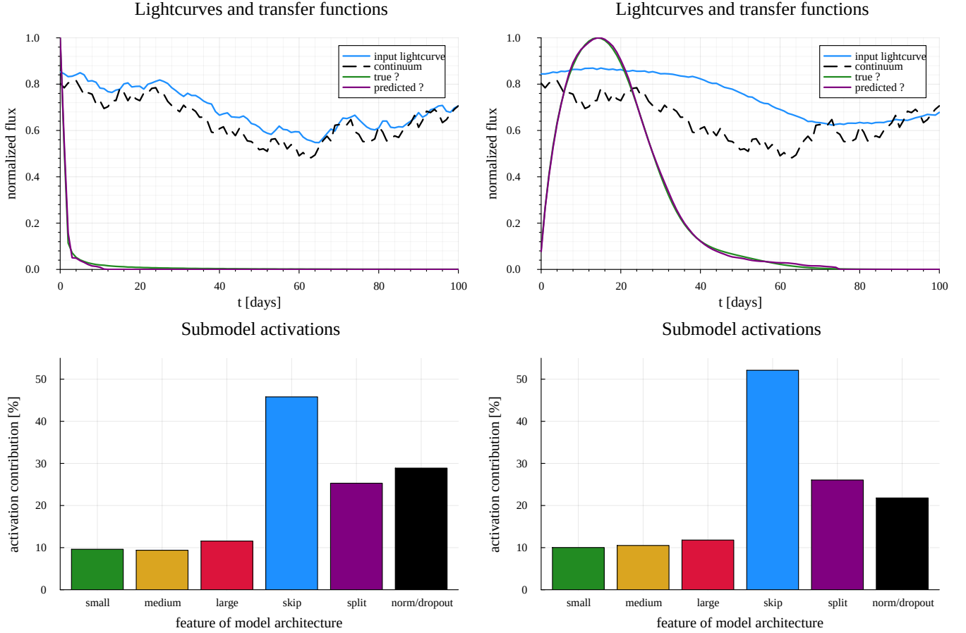
Figure 9. Here we showcase the percentage of activations (how strongly the model responds to an input and thus how much each feature contributes to the final prediction) for two very different input lightcurves. The left was generated using a transfer function with a narrow peak, and thus producing variations in the line lightcurve primarily on short timescales. The right panel shows a lightcurve generated from a transfer function that extends to much longer times, thus the lightcurve is much smoother and varies on an intrinsically longer timescale. The bottom panels of both plots show the activation percentages of various components of our model architecture. The left three bars (small, medium, and large) correspond to the sum of all activations in each of the corresponding time filters. The blue “skip” bar showcases how important the overall skip connection design is for the model, while the purple “split” bar showcases the importance of the branching path components. Finally, the black “norm/droupout” bar demonstrates the importance of the normalization and dropout layers in making the prediction. Note that thus the right three bars add up to 100% but the left three bars do not as they are subcomponents of the “skip” and “split” paths. note: this figure still in draft stage
