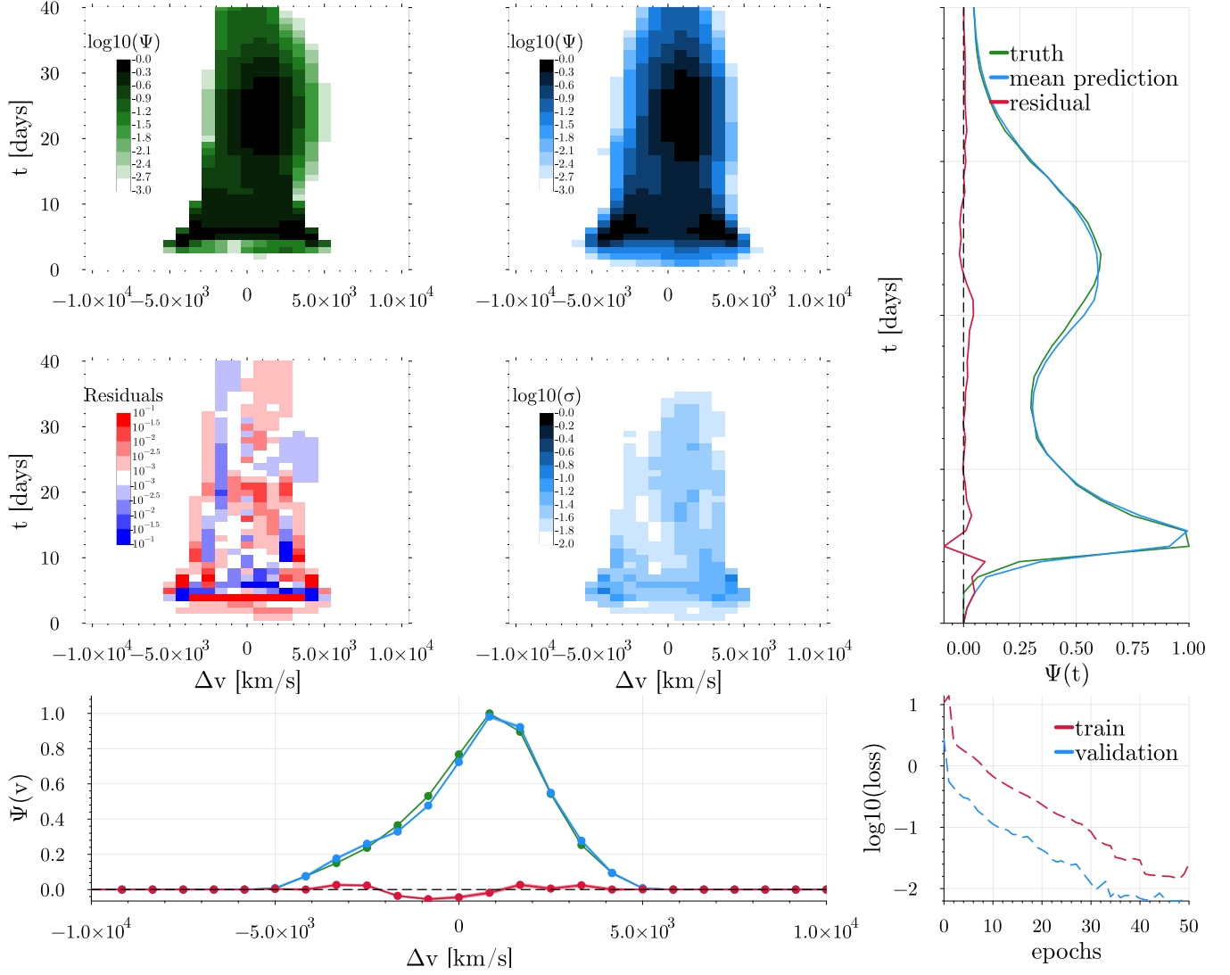
Figure 6. Top left: Sample full 2D transfer function of a complicated combined model consisting of a “disk-wind” structure with a gaussian blob of gas added at later times and offset from line center. Top middle: (D)CNN model recovery of the full 2D transfer function. Middle left: Residuals (prediction in top middle panel - ground truth shown in top left panel). The range of the colorbar shows -10% - 10% variations on an exponential scale from the maximum ground truth value. Regions where the model overpredicts are shown in red, underpredicted regions are shown in blue, and areas in white are where the model prediction is within \pm 0.1\% of the maximum ground truth power. Clearly the Keplerian disk’s ring-like structure’s sharpness in the ground truth poses some problems for the model, but overall it does quite well. Middle right: The uncertainty in the ensemble of predictions for this lightcurve. Note that the ensemble of models are most uncertain of where the edges are and how much intensity should go in the inner region, as highlighted in the residuals. Top/middle subpanel: The 1D transfer function (2D maps integrated as a function of velocity, see Figure 3) showing the mean model prediction in blue (with ribbon corresponding to uncertainty), the ground truth in green, and the residuals in red. Bottom left/middle: The 1D line profile (2D maps integrated as a function of time) again showing the mean model prediction in blue (with ribbon corresponding to the uncertainty), the ground truth in green, and the residuals in red. Bottom right: Mean loss curves for the ensemble of models, with the validation shown in blue and the training set shown in red.
