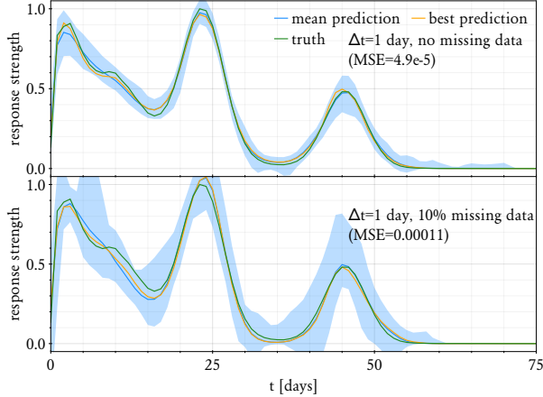
Figure 4. Comparing how the network performs when the training data quality are degraded Top: The reference network prediction for the more complicated transfer function as shown in Figure 2 trained on perfectly sampled data. bottom: Sample recovery of the more complicated transfer function formed from the combination of several of the basis transfer functions shown in Figure 2, but this time from a set of models trained with random observational gaps.
