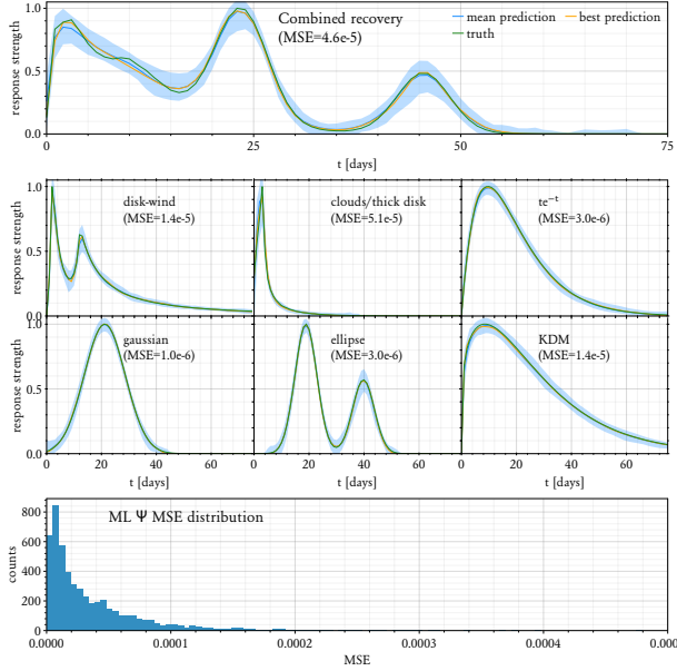
Figure 3. Top: Sample recovery of a more complicated transfer function formed from the combination of several of the basis transfer functions shown in Figure 2. Middle: Sample recoveries of each of the six “basis” transfer functions. Bottom: Distribution of errors for model predictions.
