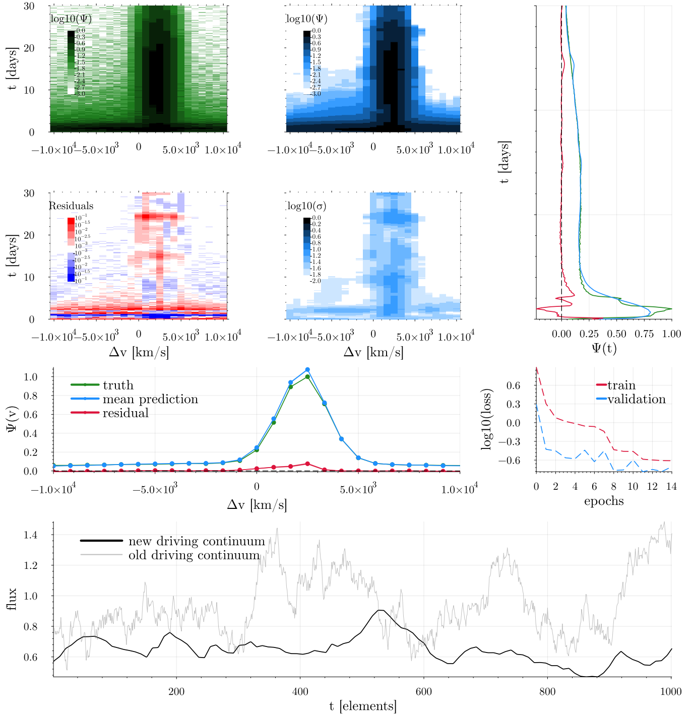
Figure 7. A 2D inversion of another complicated combined transfer function, this time the result of a physical cloud distribution confined to close distances and an elongated gaussian cloud distribution off line center. The prediction was generated using an ensemble of models fine-tuned for just 14 additional epochs (starting from the parameters used in generating the inversions shown in Figure 6 and with the same plot panels as described in the caption there). As shown in the bottom panel the continuum lightcurve and training datasets used for the fine-tuning were completely different in this case, with a significantly reduced physical timescale ( \sim 100 days instead of \sim 1000 days) and more poorly resolved variations.
