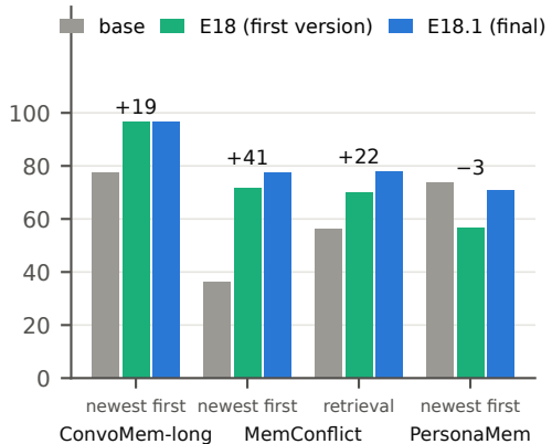
(b) Dated list in thinking (held-out sets)
