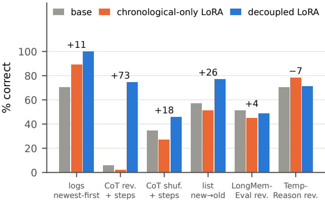
(a) Selection: decoupled training (answer only)
