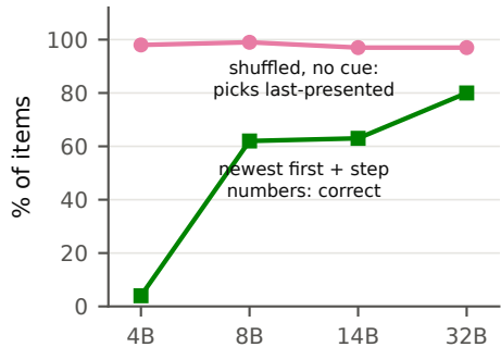
(b) Chains of thought, k = 8 overwrites
