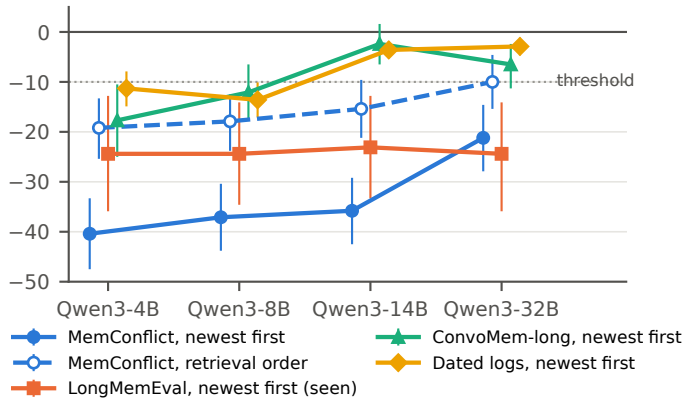
(a) Order effect on memory questions, by model size
