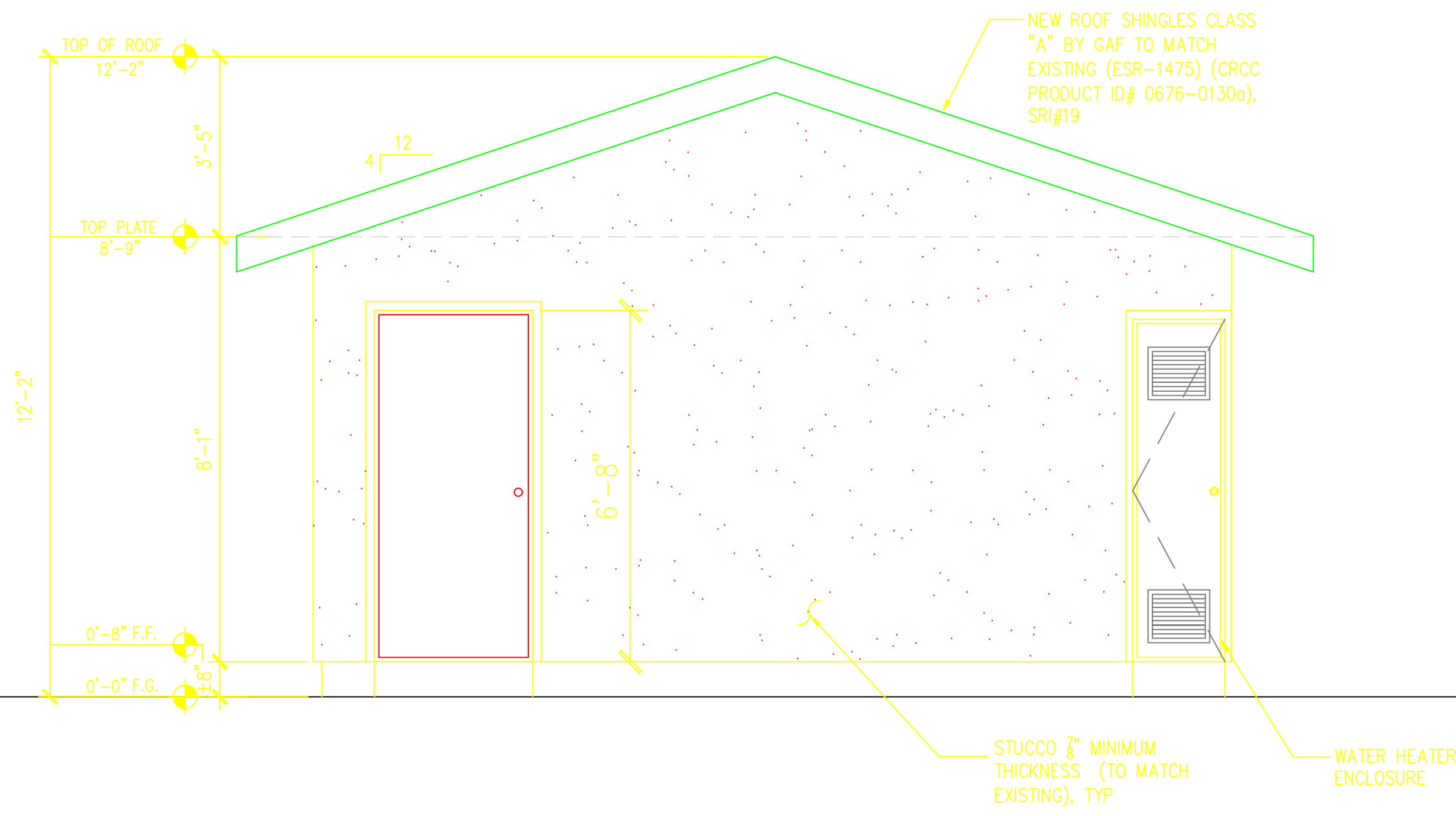
PROPOSED SOUTH ELEVATION 3/8 = 1'-0"
