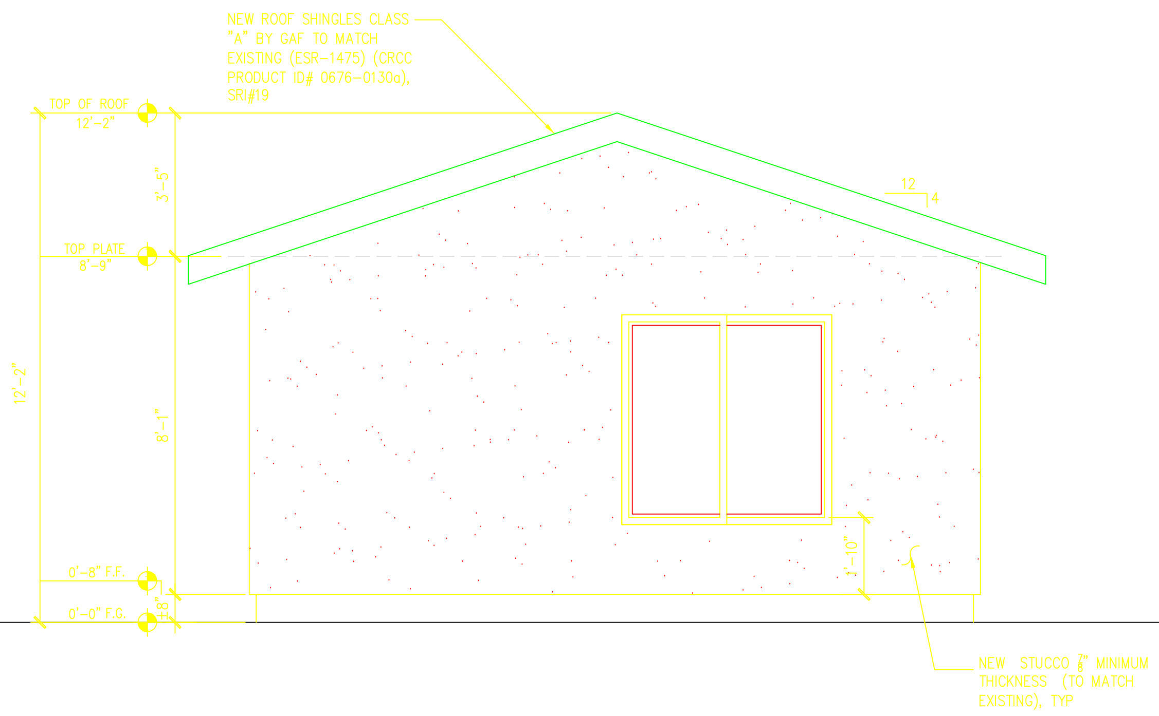
PROPOSED NORTH ELEVATION 3/8 = 1'-0"
