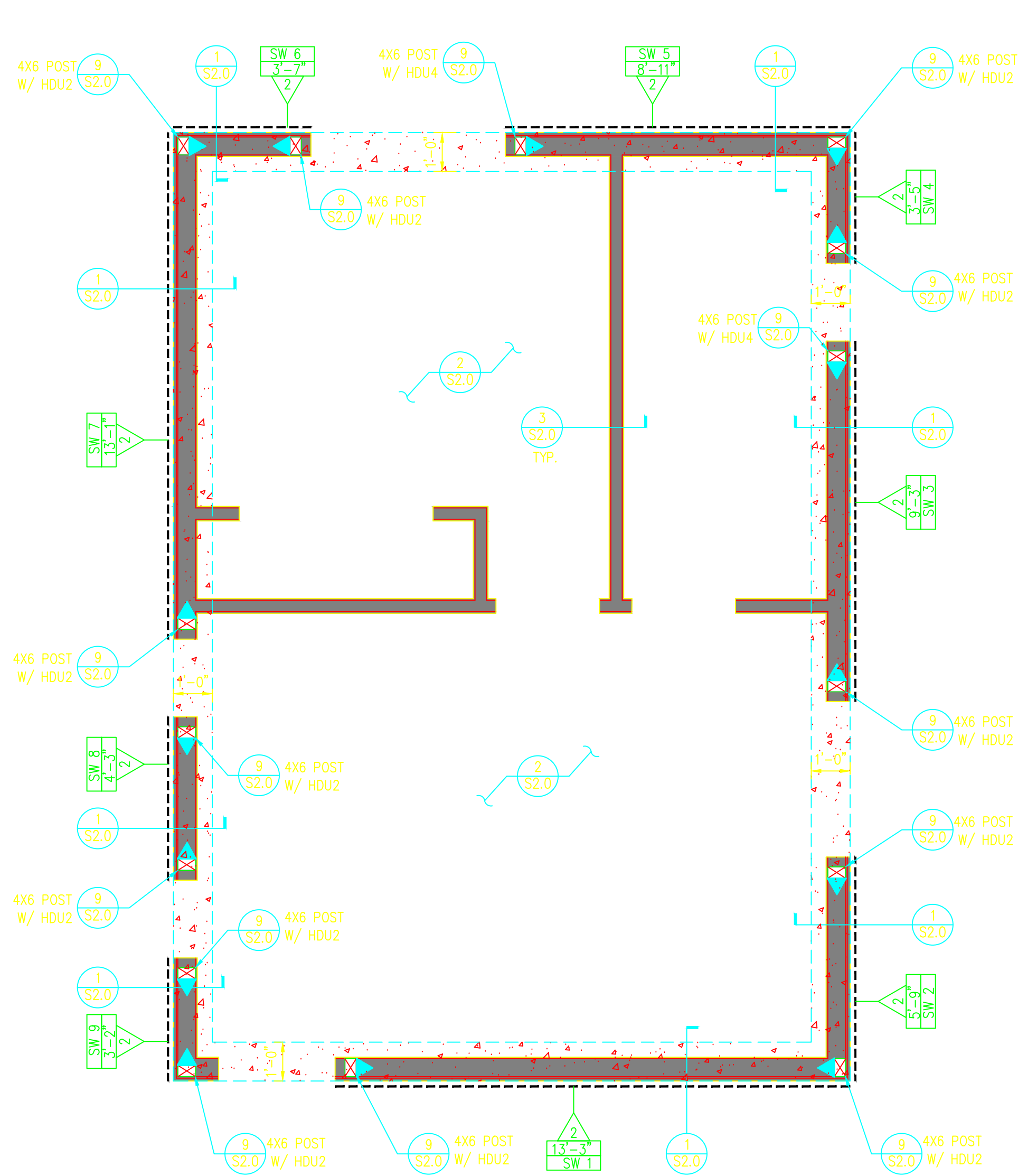
FOUNDATION PLAN 3/8" = 1'-0"
