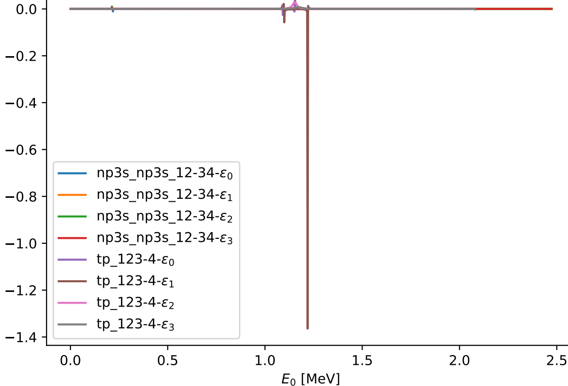
a_{dd} dependence on E_0
