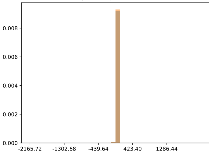
max(variance) = 7424.248855
