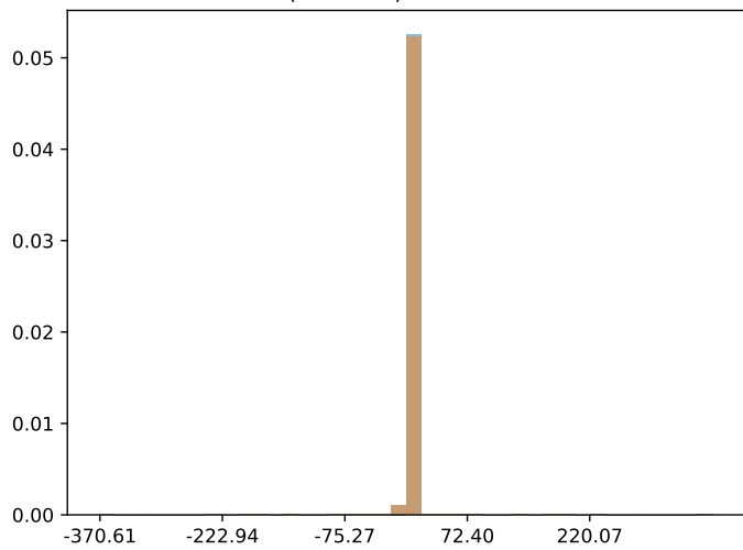
max(variance) = 250.759943
