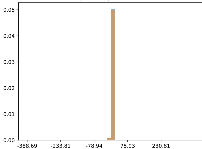
max(variance) = 268.125957
