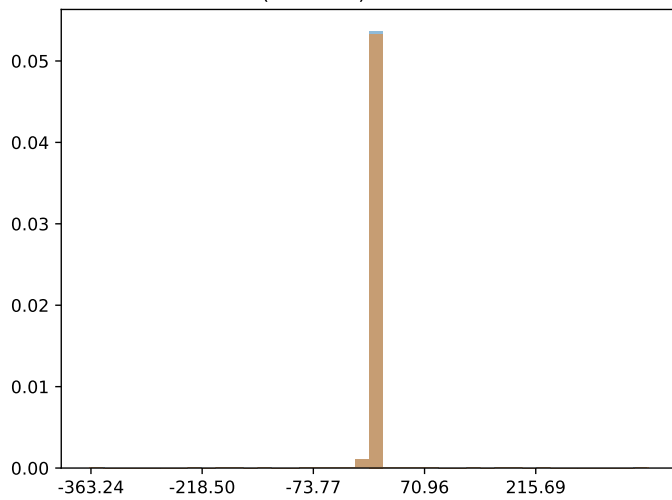
max(variance) = 244.479715
