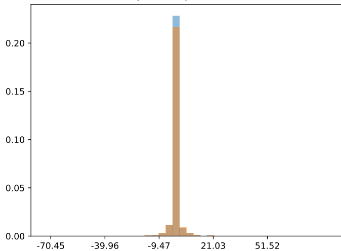
max(variance) = 26.717984
