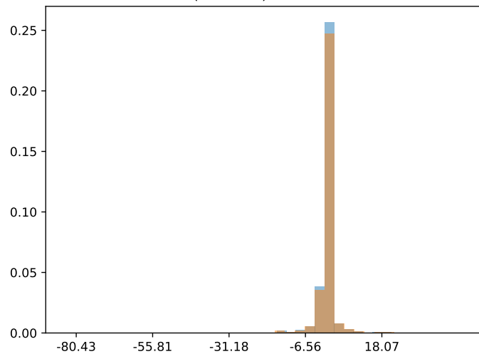
max(variance) = 22.326215
