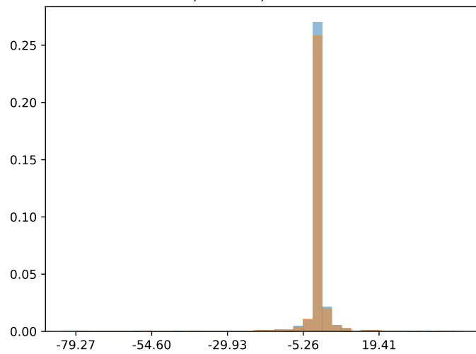
max(variance) = 22.817363
