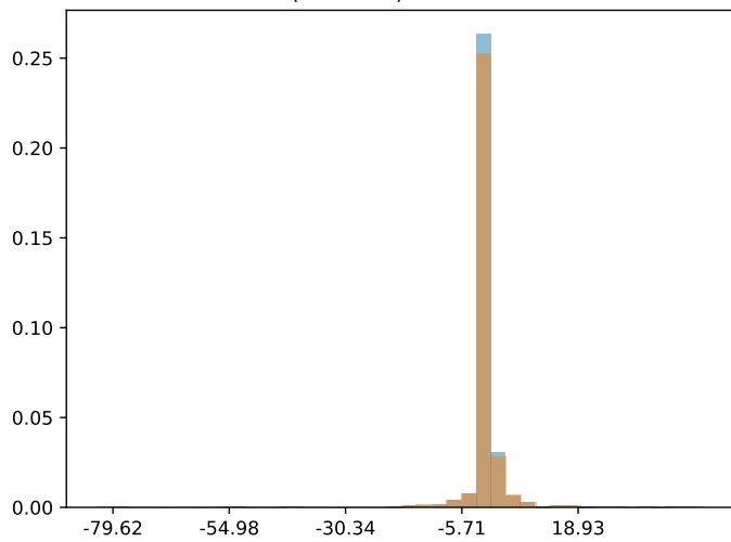
max(variance) = 22.671472
