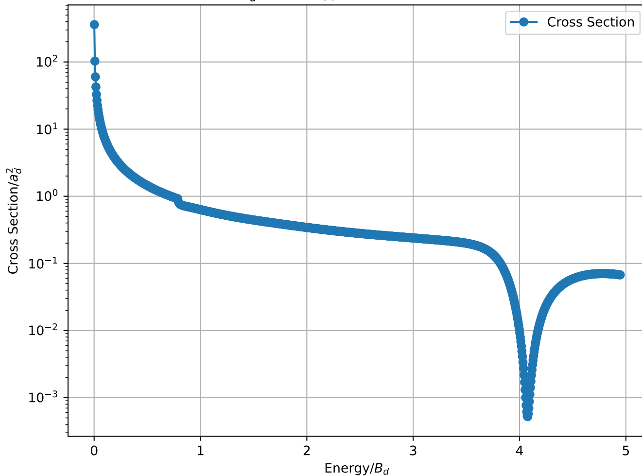
Cross Section/ a_d^2 vs Energy/ B_d for 1-1 B_3 = 1.04 MeV , L=8
