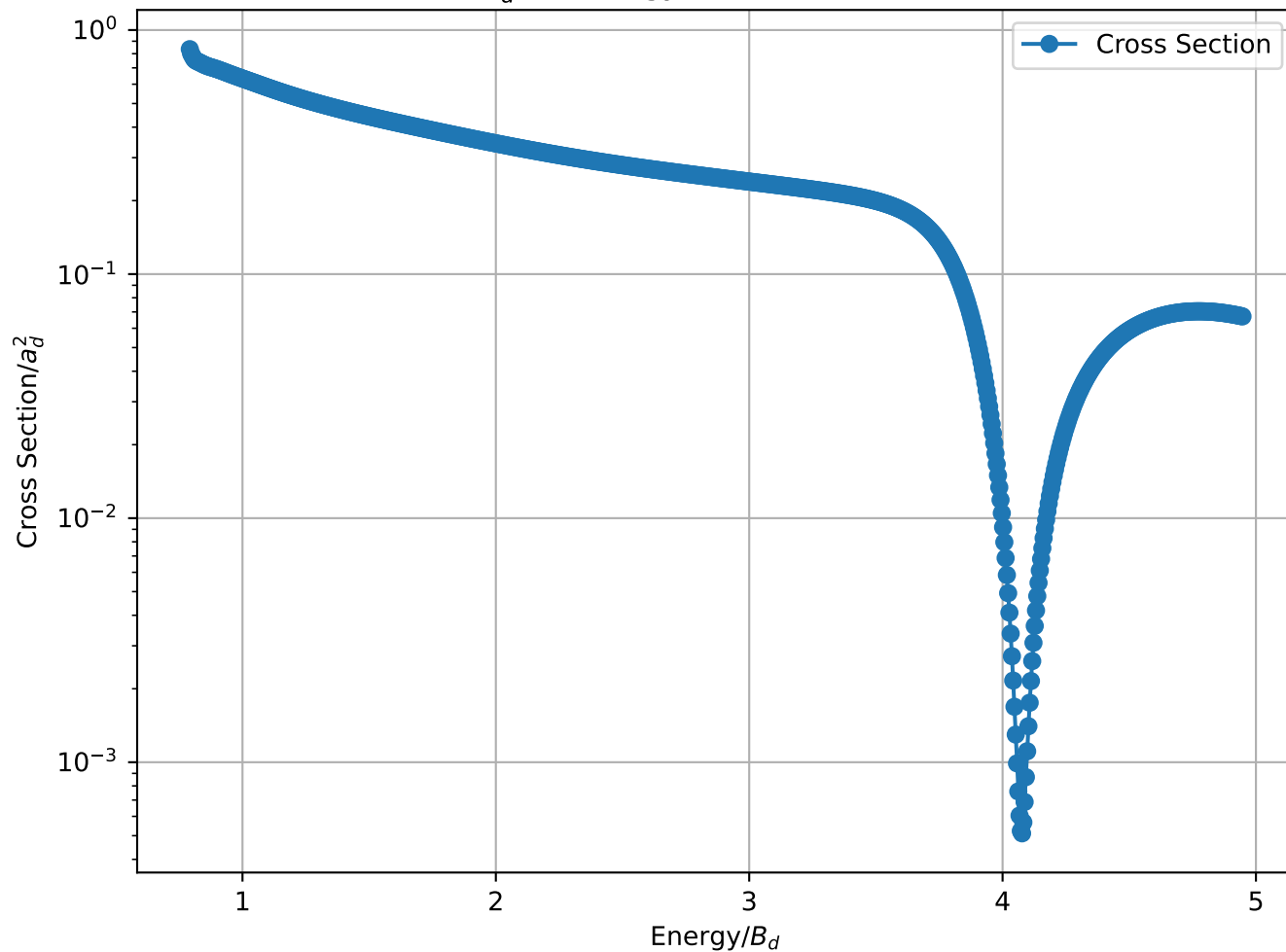
Cross Section/ a_d^2 vs Energy/ B_d for 2-2 B_3 = 1.04 MeV , L=8
