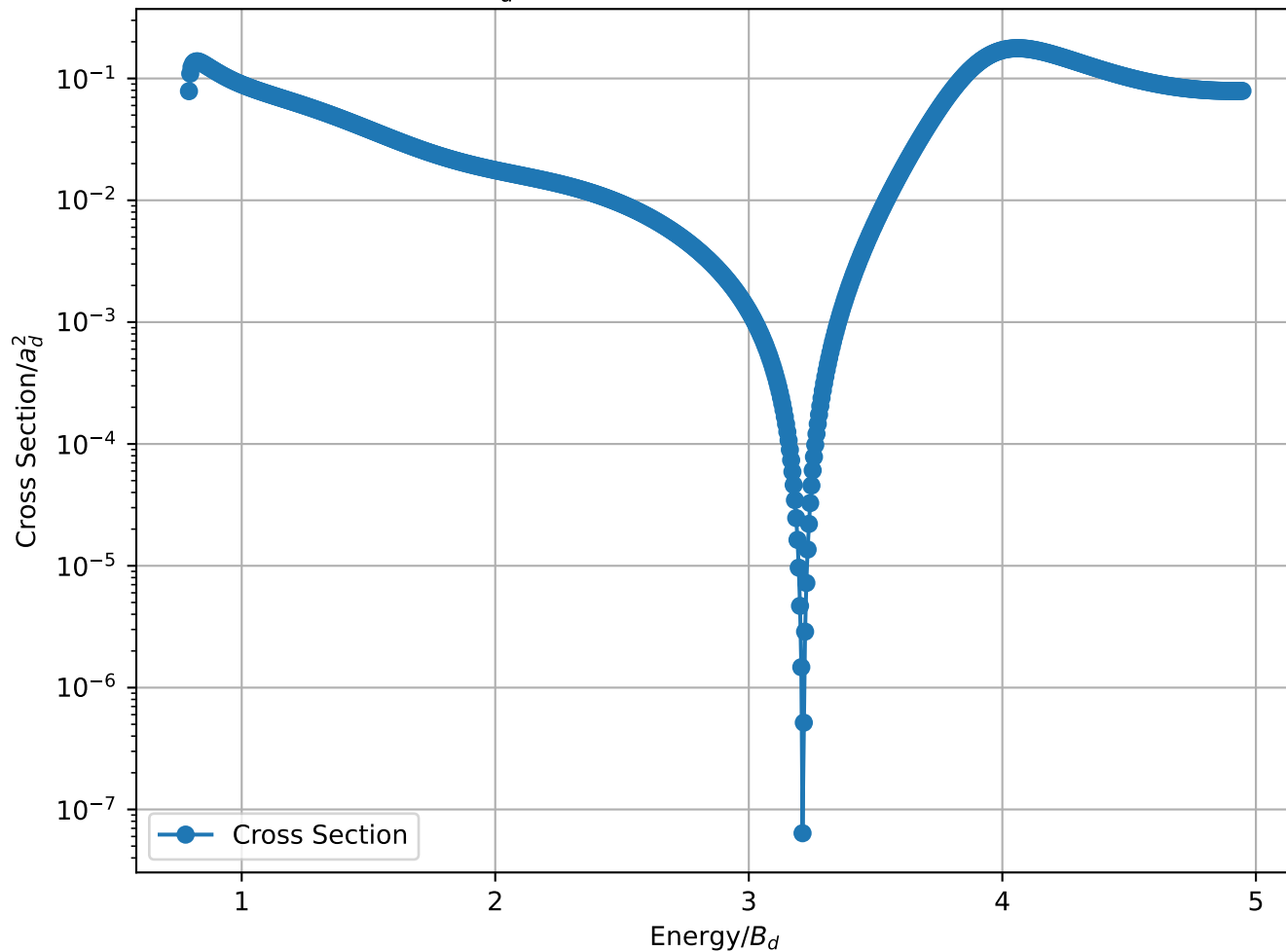
Cross Section/ a_d^2 vs Energy/ B_d for 1-2 B_3 = 1.04 MeV , L=8
