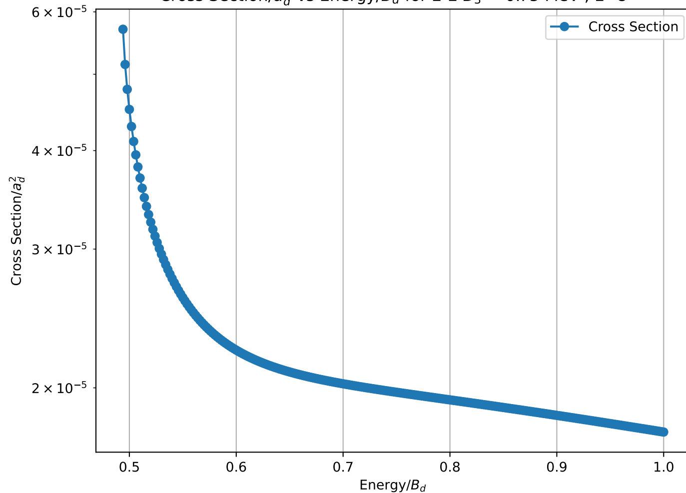
Cross Section/ a_d^2 vs Energy/ B_d for 2-2 B_3 = 0.75 MeV , L=8
