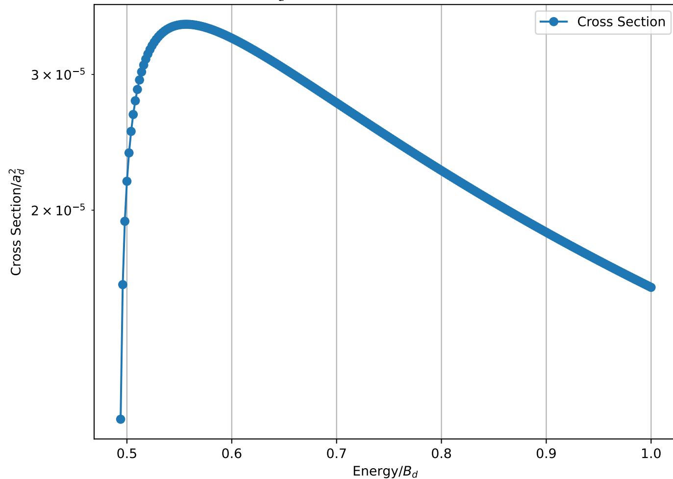
Cross Section/ a_d^2 vs Energy/ B_d for 1-2 B_3 = 0.75 MeV , L=8
