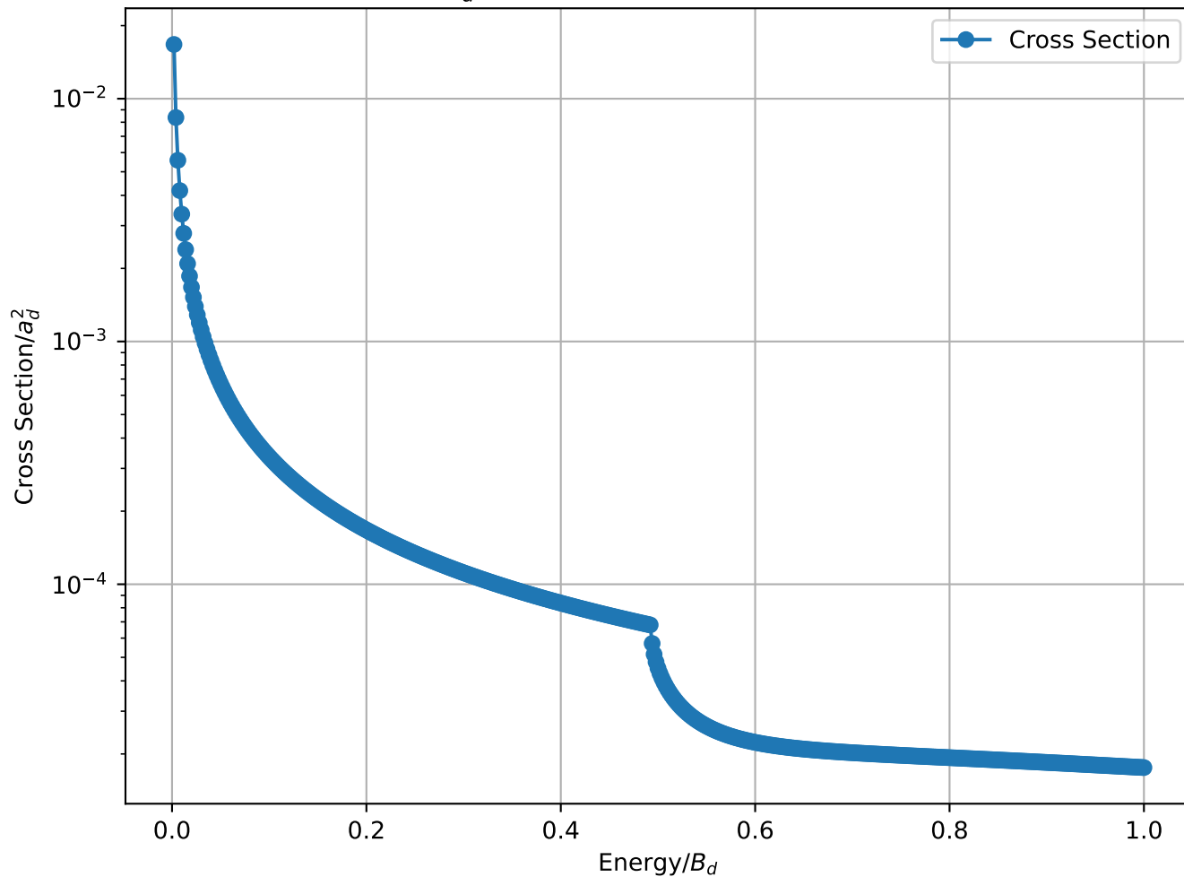
Cross Section/ a_d^2 vs Energy/ B_d for 1-1 B_3 = 0.75 MeV , L=8
