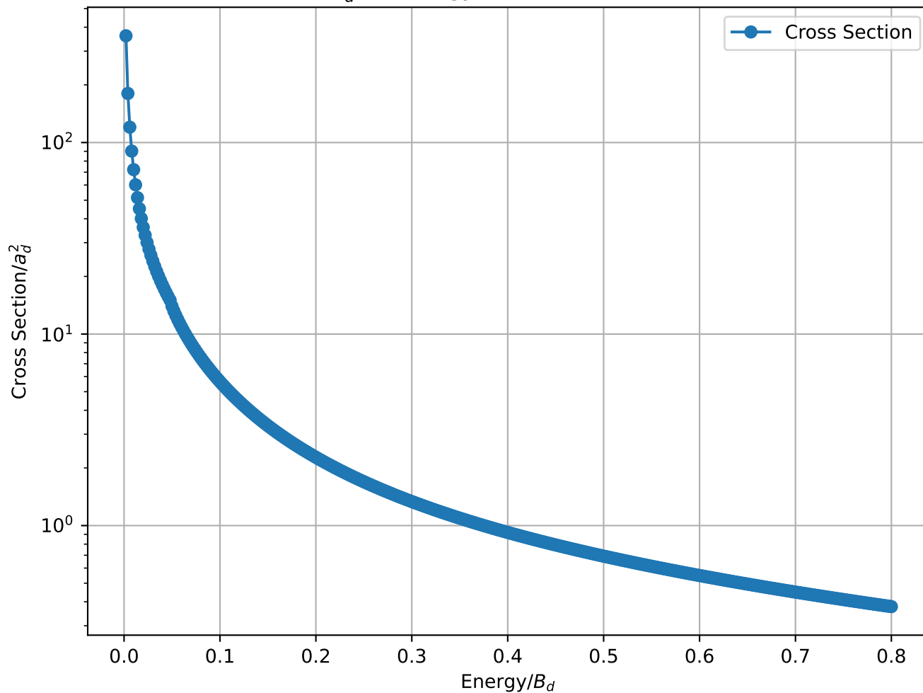
Cross Section/ a_d^2 vs Energy/ B_d for 1-1 B_3 = 0.96 MeV , L=10
