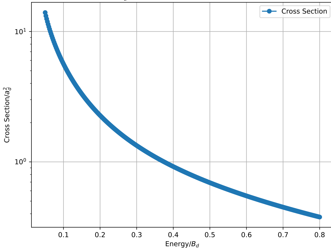
Cross Section/ a_d^2 vs Energy/ B_d for 2-2 B_3 = 0.96 MeV , L=10
