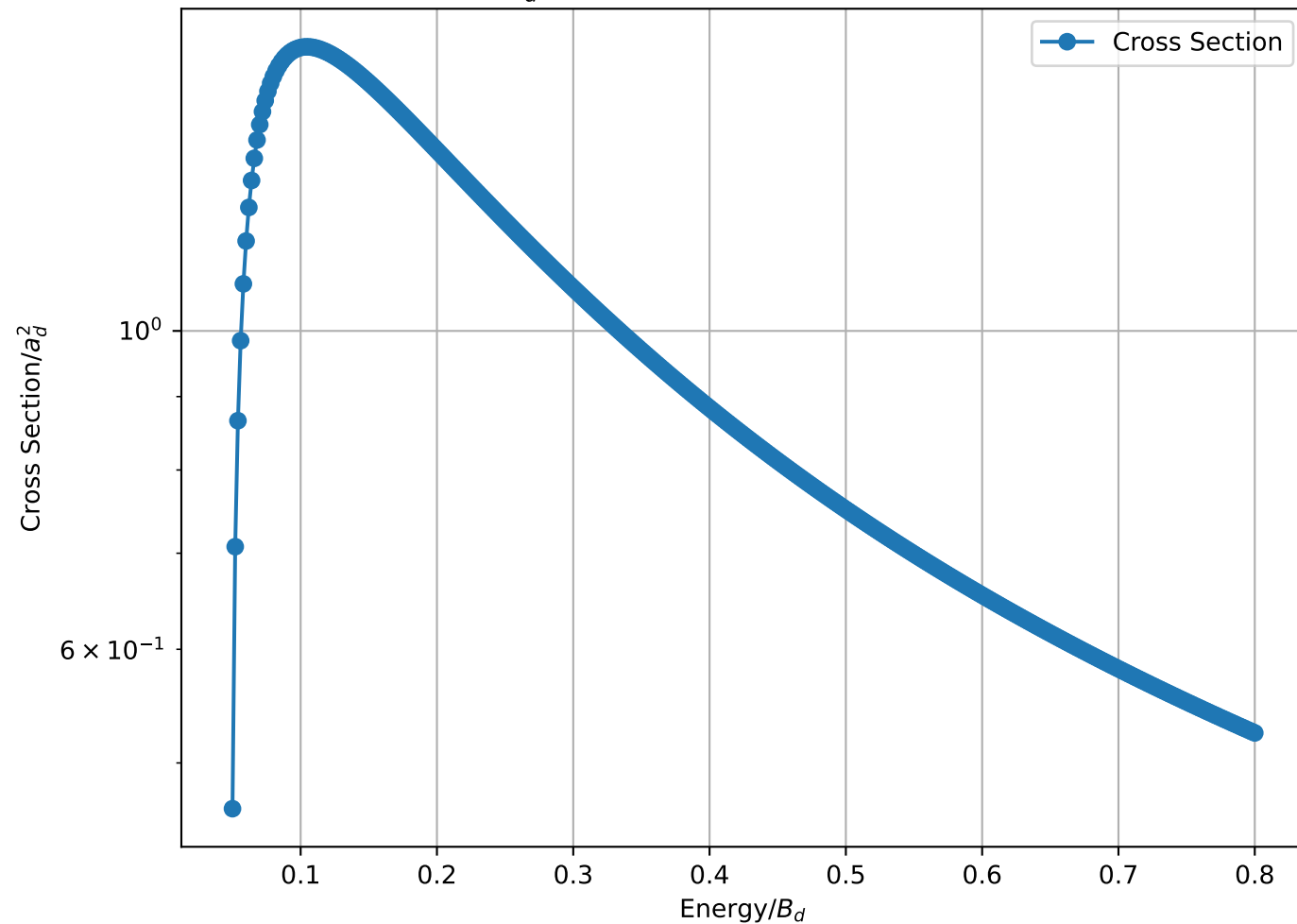
Cross Section/ a_d^2 vs Energy/ B_d for 1-2 B_3 = 0.96 MeV , L=10
