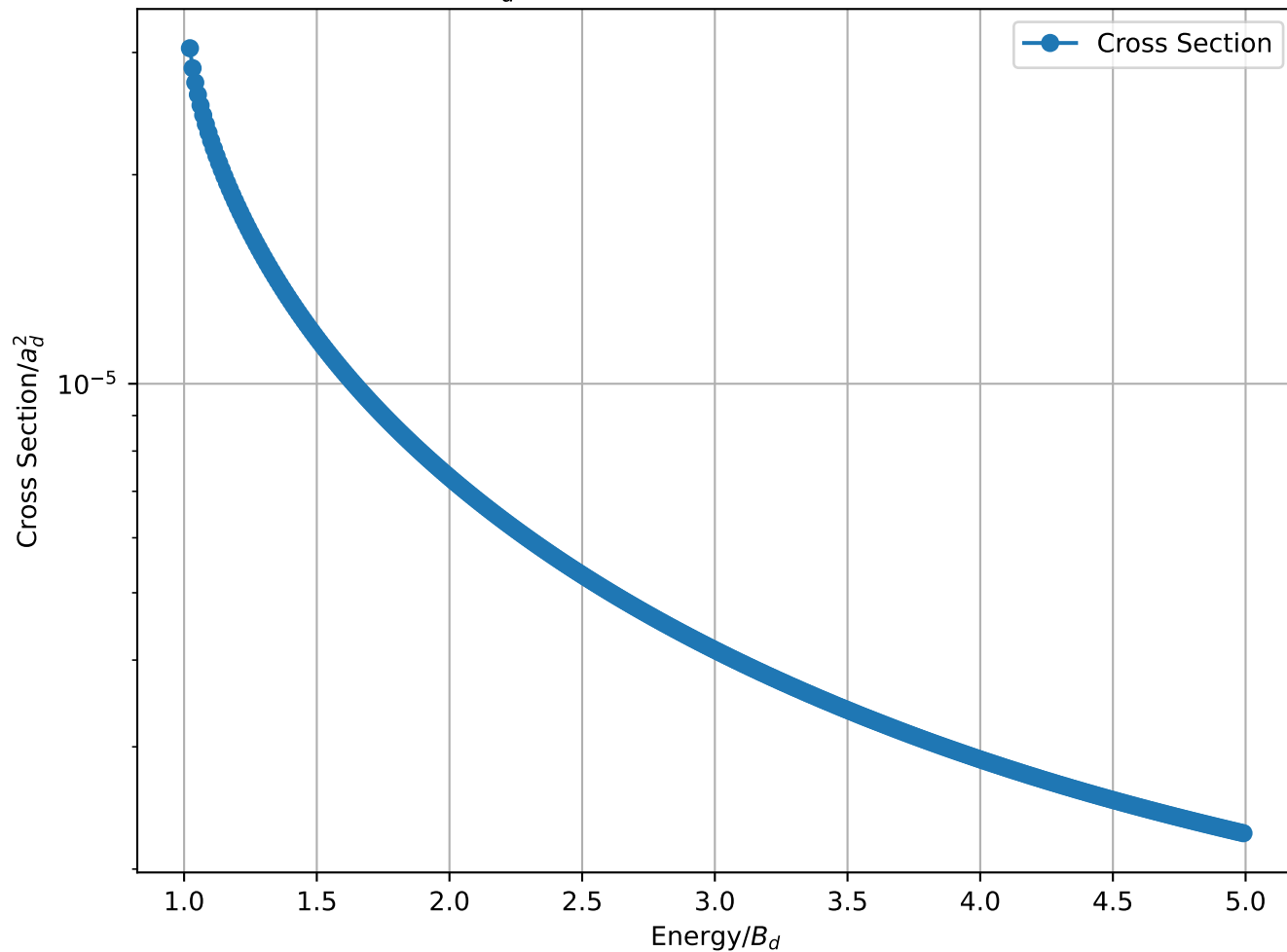
Cross Section/ a_d^2 vs Energy/ B_d for 2-2 B_3 = 1.50 MeV , L=6
