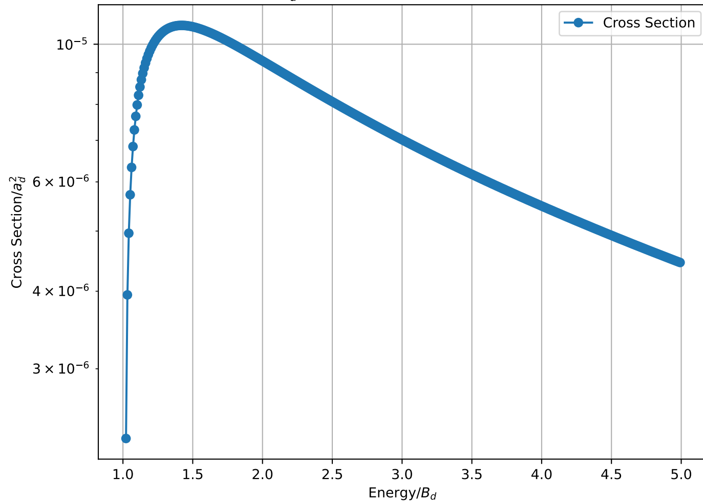
Cross Section/ a_d^2 vs Energy/ B_d for 1-2 B_3 = 1.50 MeV , L=6
