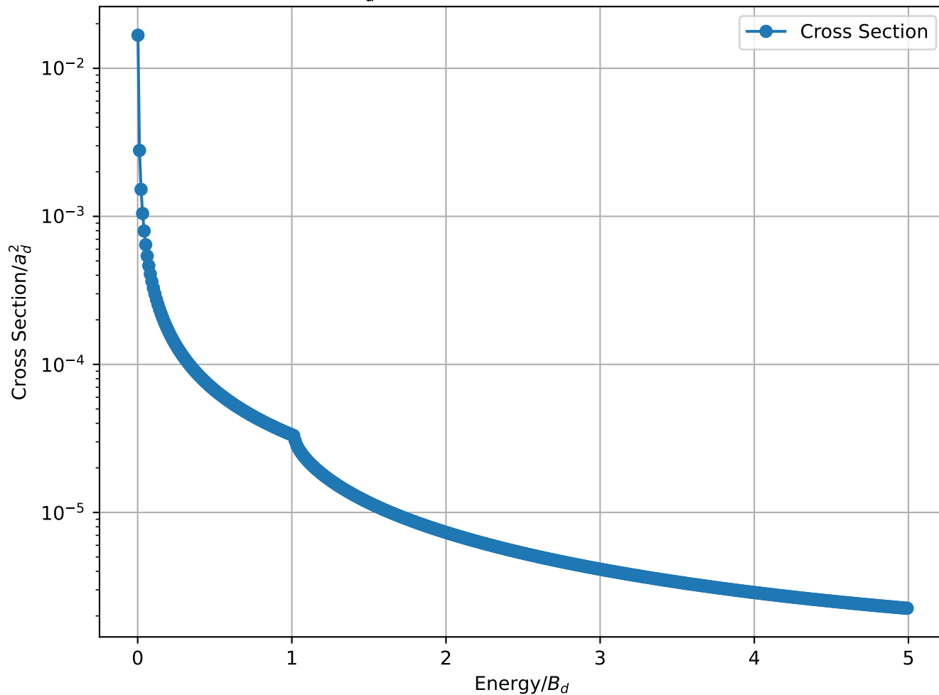
Cross Section/ a_d^2 vs Energy/ B_d for 1-1 B_3 = 1.50 MeV , L=6
