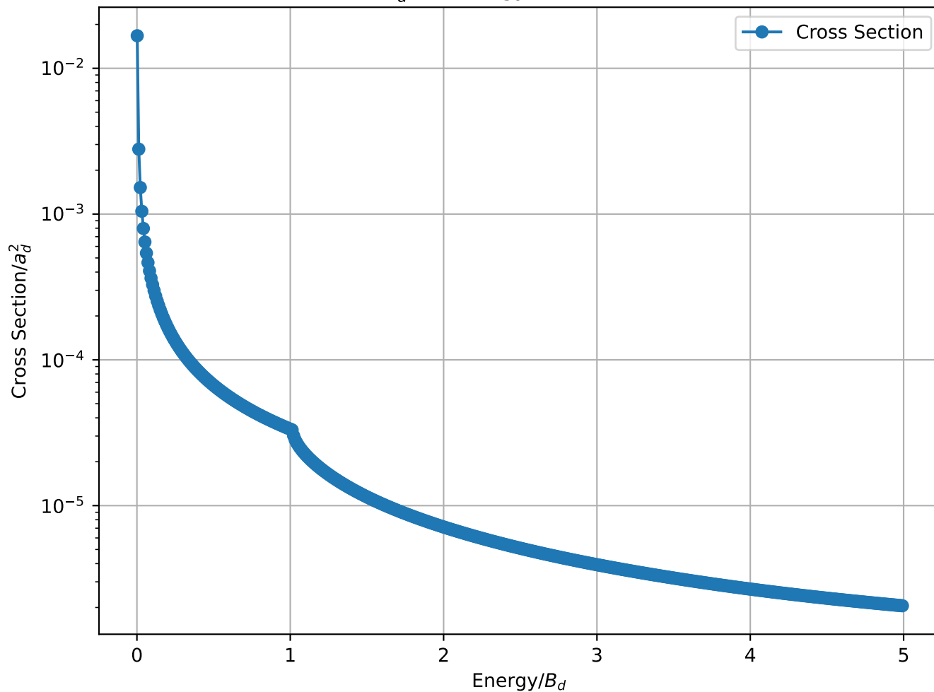
Cross Section/ a_d^2 vs Energy/ B_d for 1-1 B_3 = 1.50 MeV
