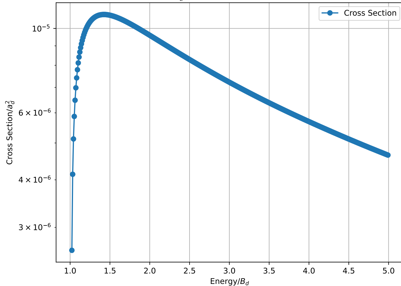
Cross Section/ a_d^2 vs Energy/ B_d for 1-2 B_3 = 1.50 MeV
