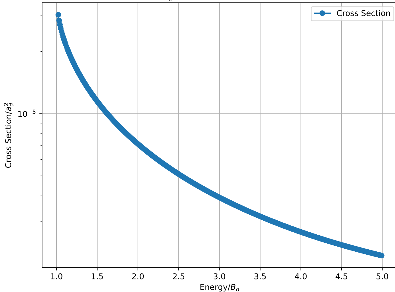
Cross Section/ a_d^2 vs Energy/ B_d for 2-2 B_3 = 1.50 MeV
