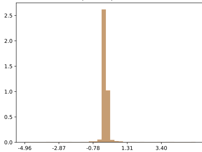
max(variance) = 0.085390
