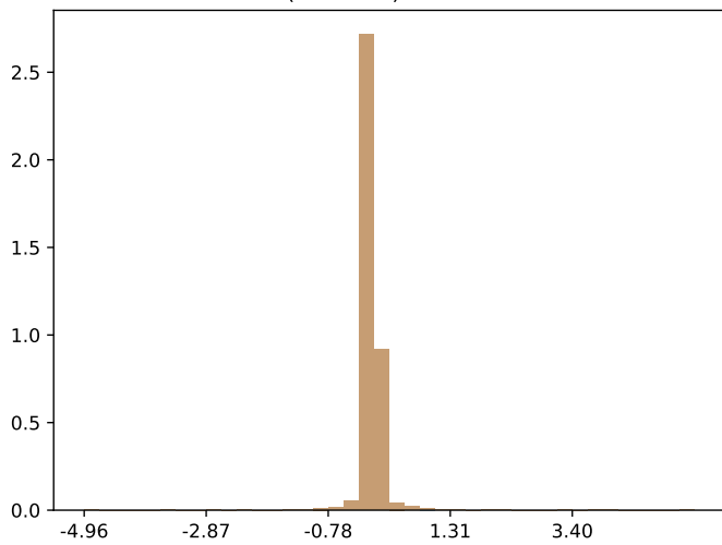
max(variance) = 0.085625
