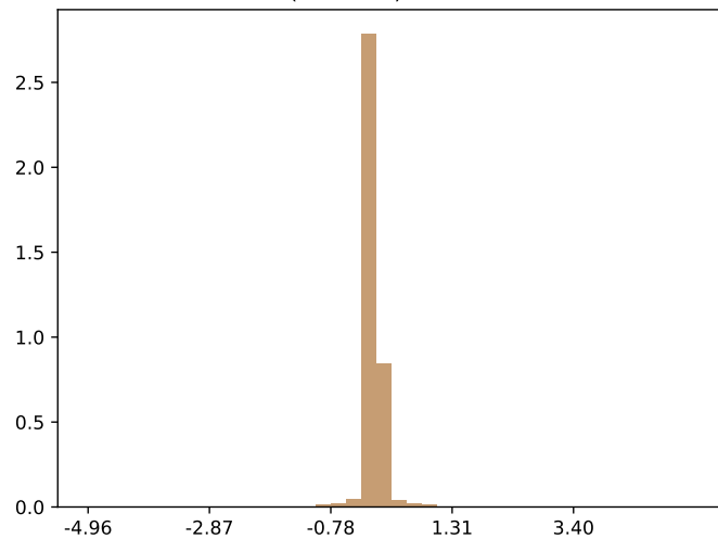
max(variance) = 0.085930
