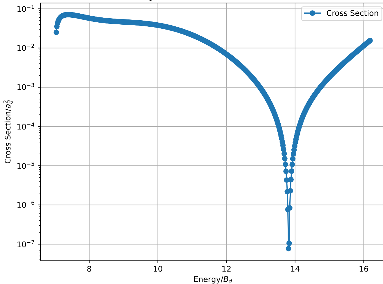
Cross Section/ a_d^2 vs Energy/ B_d for 1-2 B_3 = 4.50 MeV , L=4
