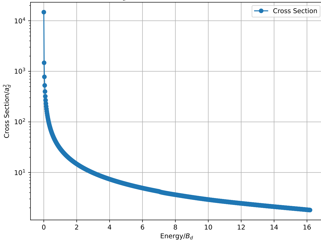
Cross Section/ a_d^2 vs Energy/ B_d for 1-1 B_3 = 4.50 MeV , L=4
