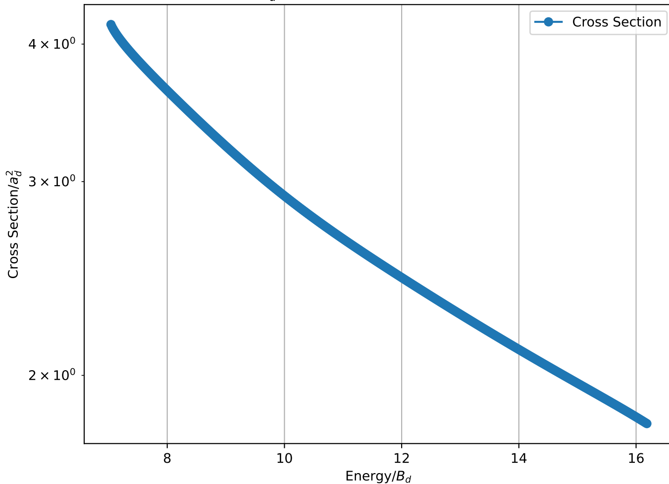
Cross Section/ a_d^2 vs Energy/ B_d for 2-2 B_3 = 4.50 MeV , L=4
