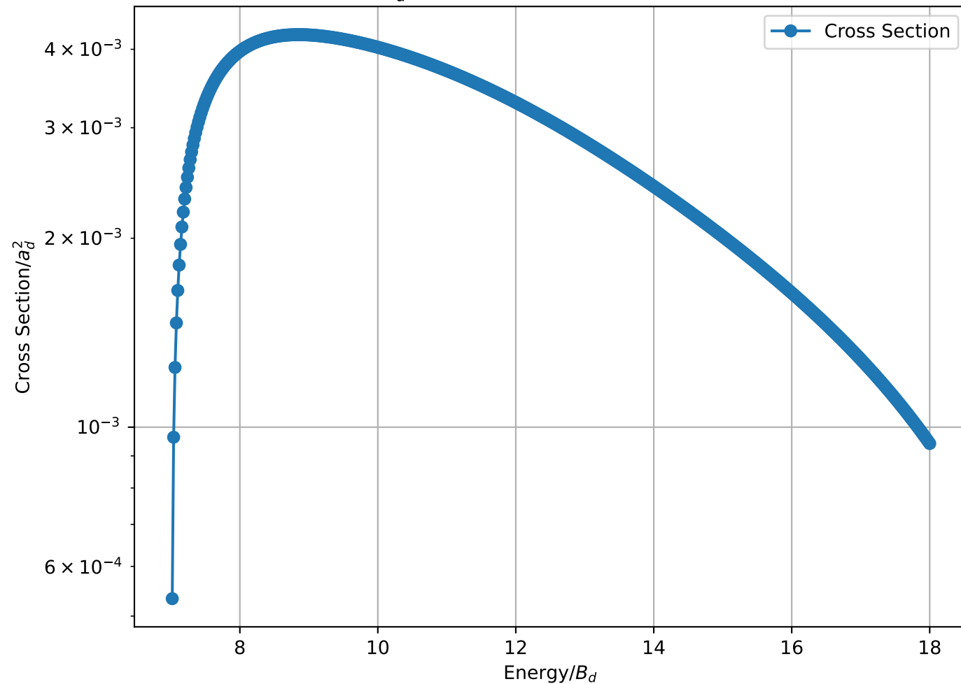
Cross Section/ a_d^2 vs Energy/ B_d for 1-2 B_3 = 1.04 MeV , L=8
