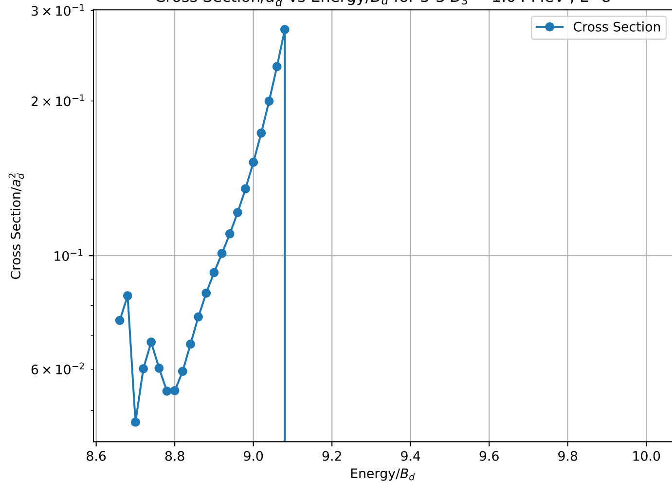
Cross Section/ a_d^2 vs Energy/ B_d for 3-3 B_3 = 1.04 MeV , L=8
