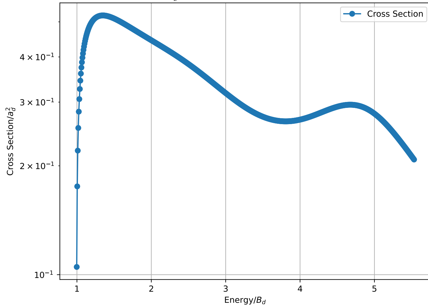
Cross Section/ a_d^2 vs Energy/ B_d for 1-2 B_3 = 3.00 MeV , L=10
