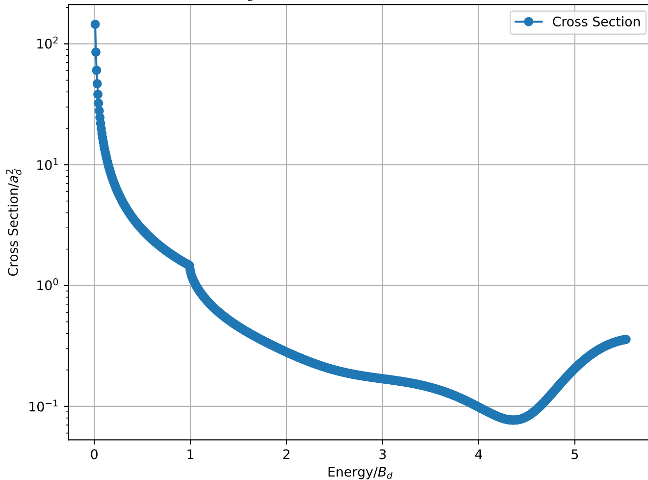
Cross Section/ a_d^2 vs Energy/ B_d for 1-1 B_3 = 3.00 MeV , L=10
