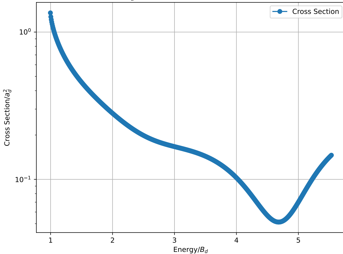
Cross Section/ a_d^2 vs Energy/ B_d for 2-2 B_3 = 3.00 MeV , L=10
