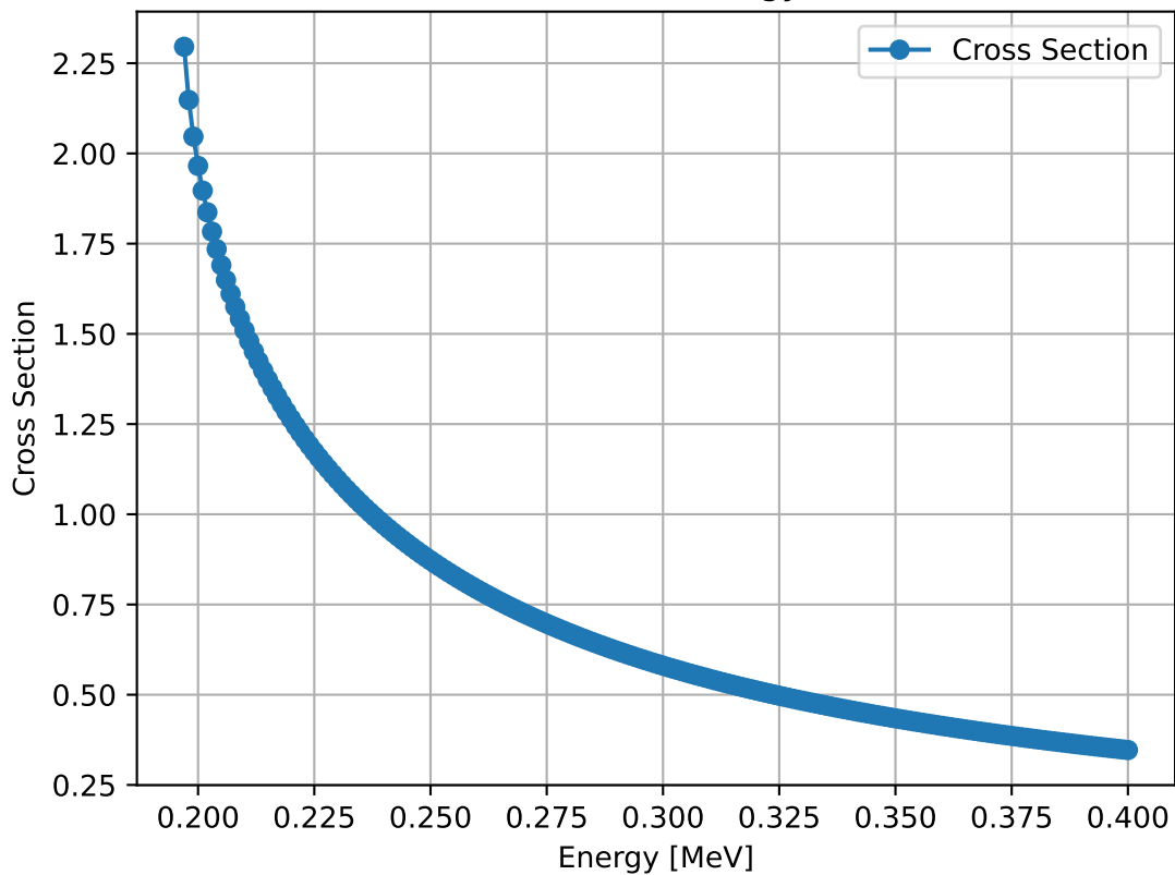
Cross Section vs Energy for 2-2
