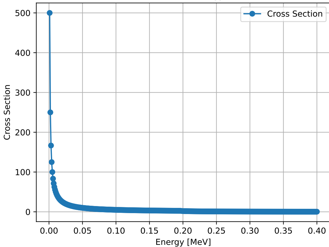
Cross Section vs Energy for 1-1
