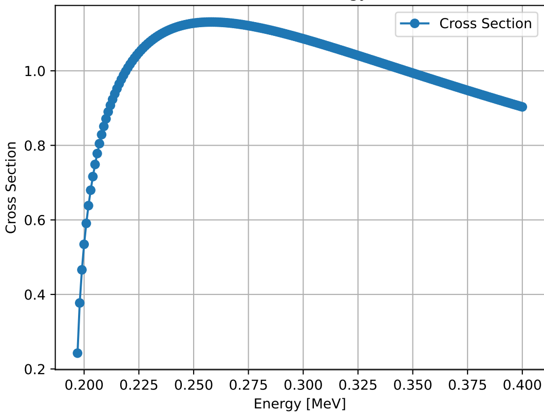
Cross Section vs Energy for 1-2
