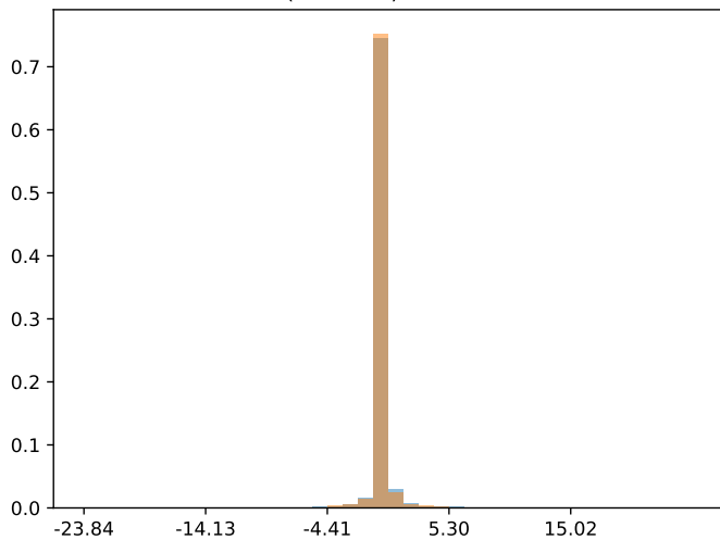
max(variance) = 2.227373
