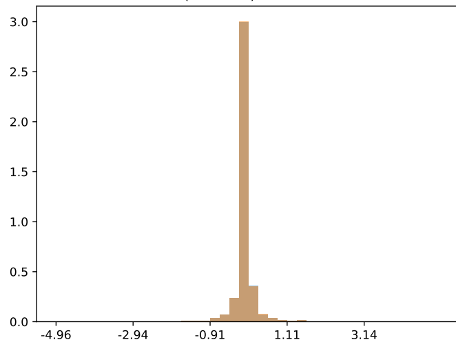
max(variance) = 0.175186
