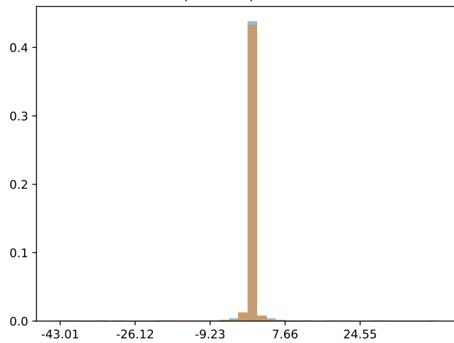
max(variance) = 6.943773
