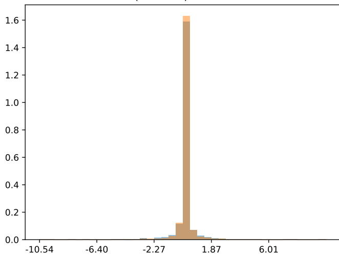
max(variance) = 0.647316
