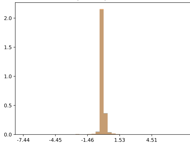
max(variance) = 0.169451
