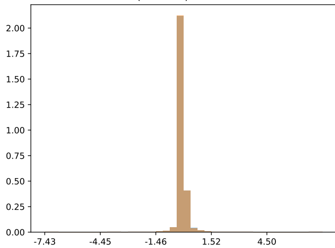
max(variance) = 0.162571
