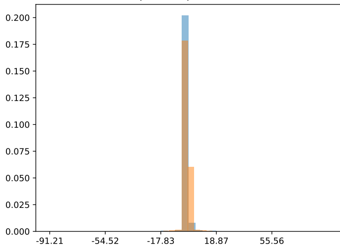
max(variance) = 39.473160
