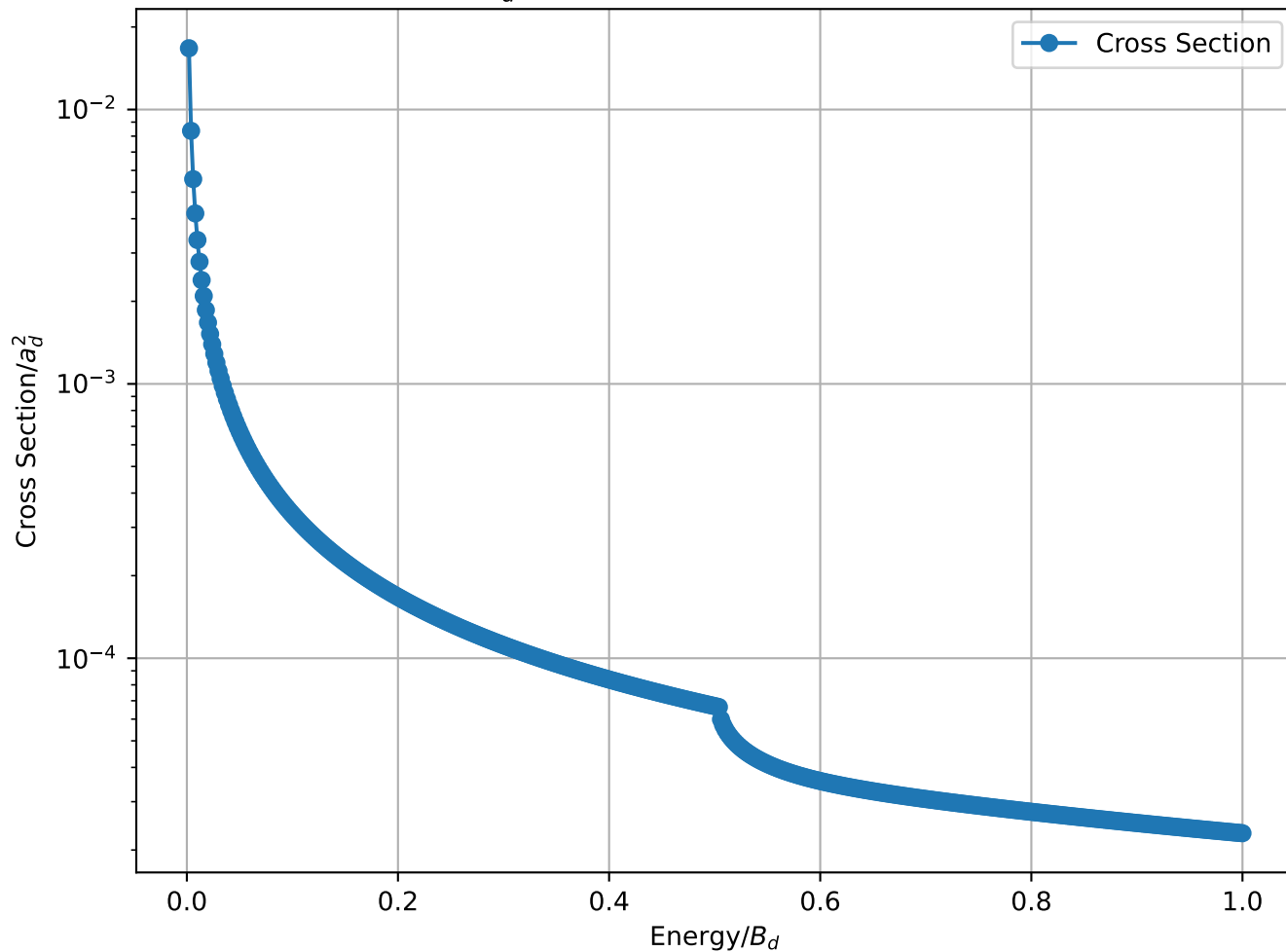
Cross Section/ a_d^2 vs Energy/ B_d for 1-1 B_3 = 0.75 MeV , L=6
