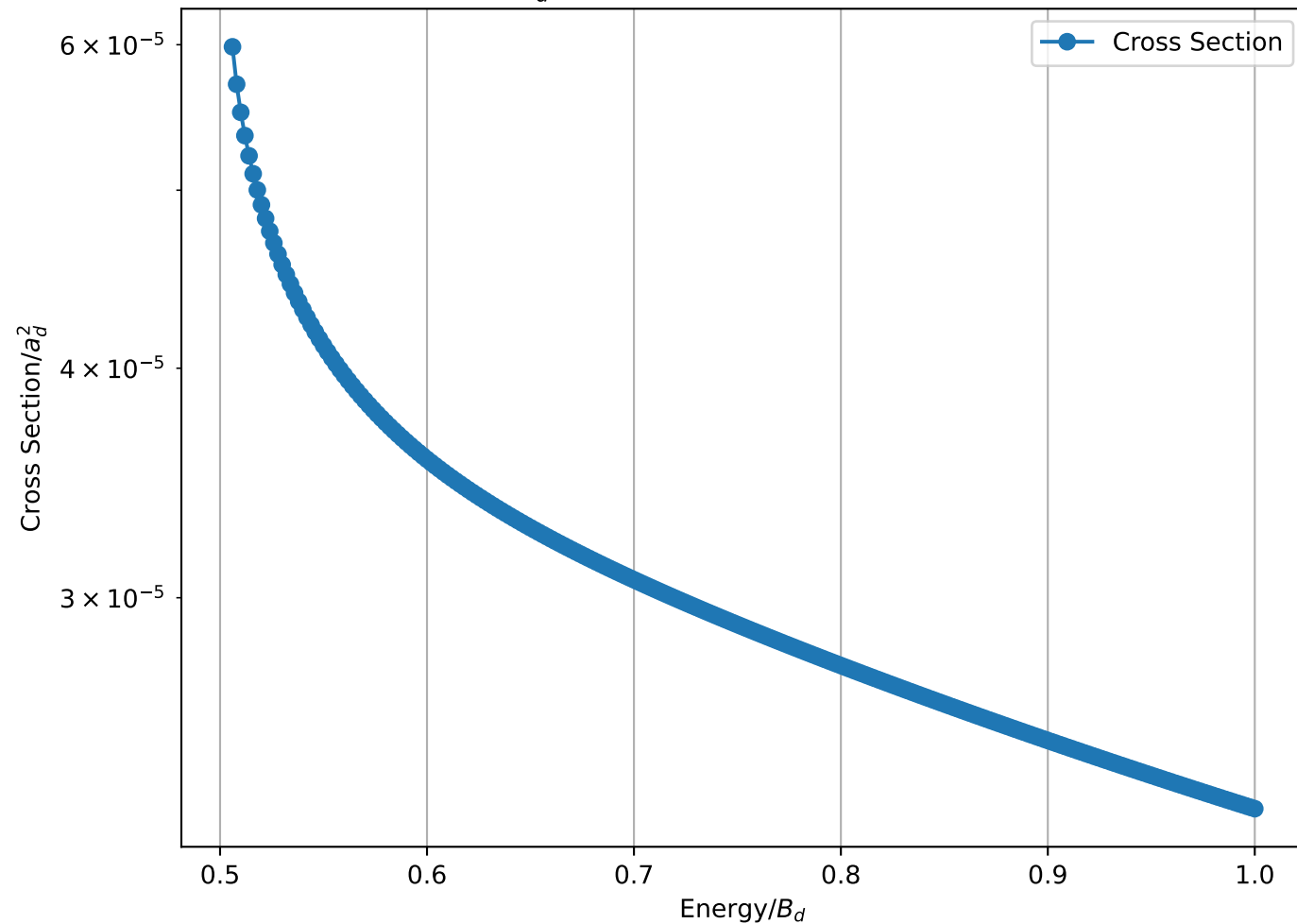
Cross Section/ a_d^2 vs Energy/ B_d for 2-2 B_3 = 0.75 MeV , L=6
