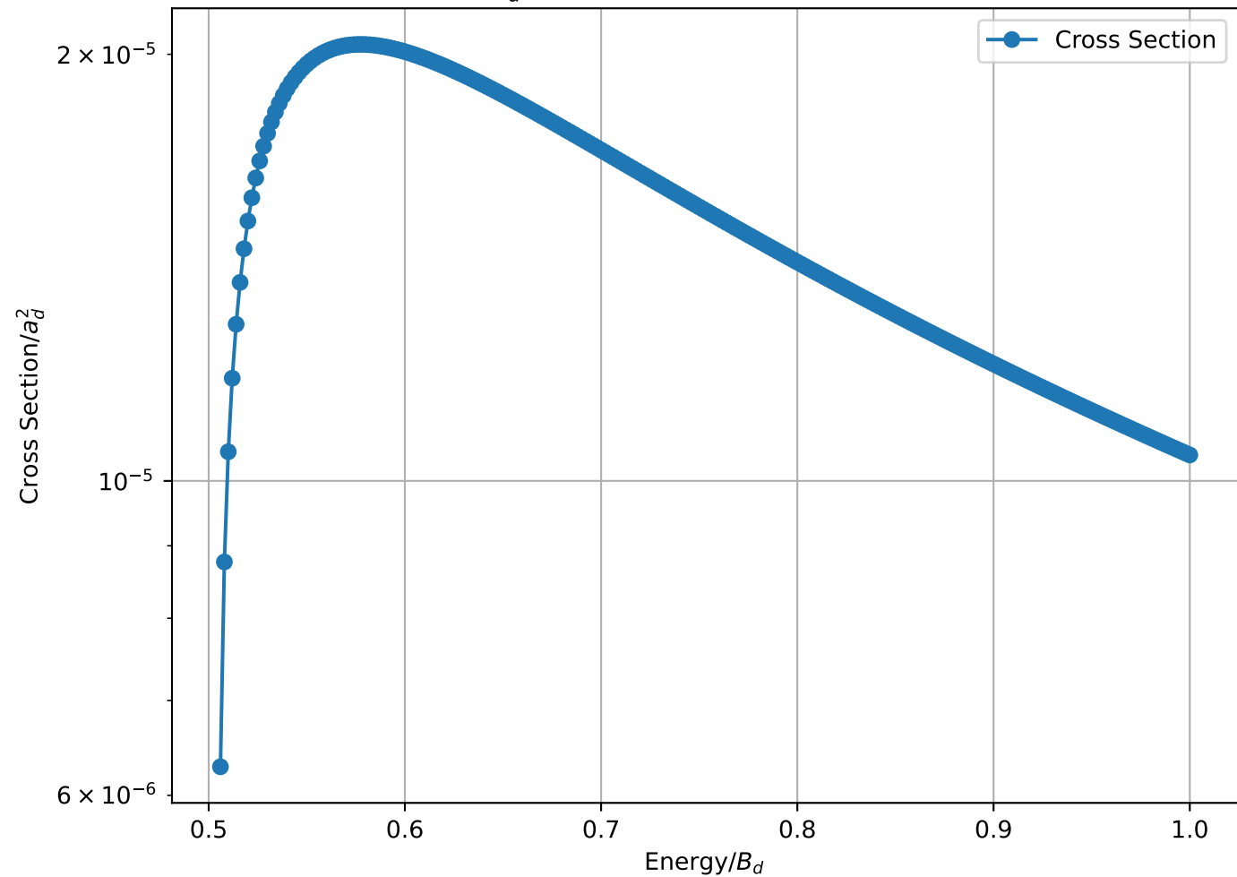
Cross Section/ a_d^2 vs Energy/ B_d for 1-2 B_3 = 0.75 MeV , L=6
