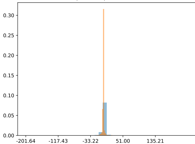
max(variance) = 128.907851
