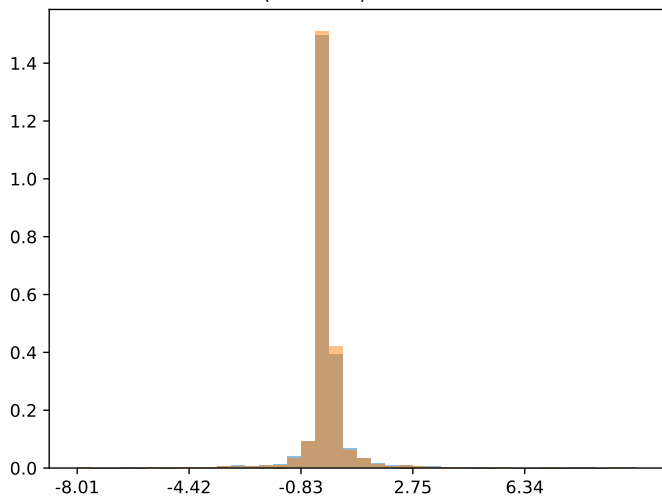
max(variance) = 0.632654
