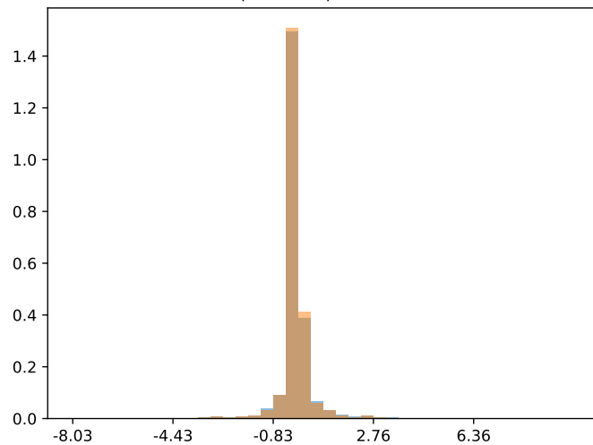
max(variance) = 0.635415
