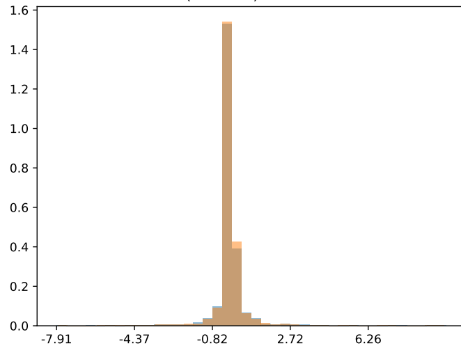
max(variance) = 0.589533
