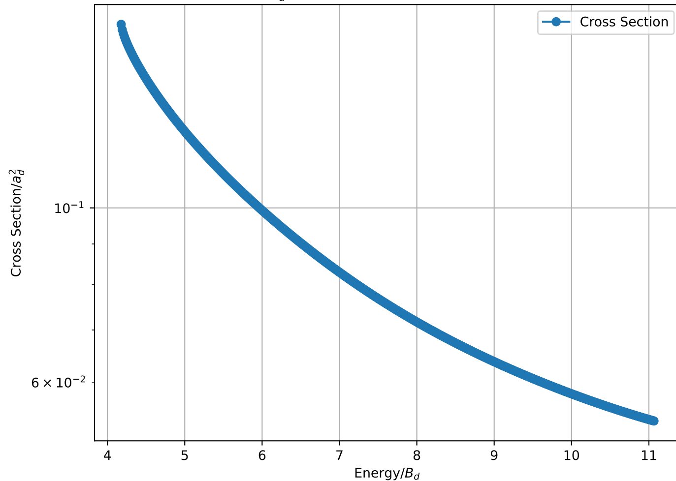
Cross Section/ a_d^2 vs Energy/ B_d for 2-2 B_3 = 1.04 MeV , L=8
