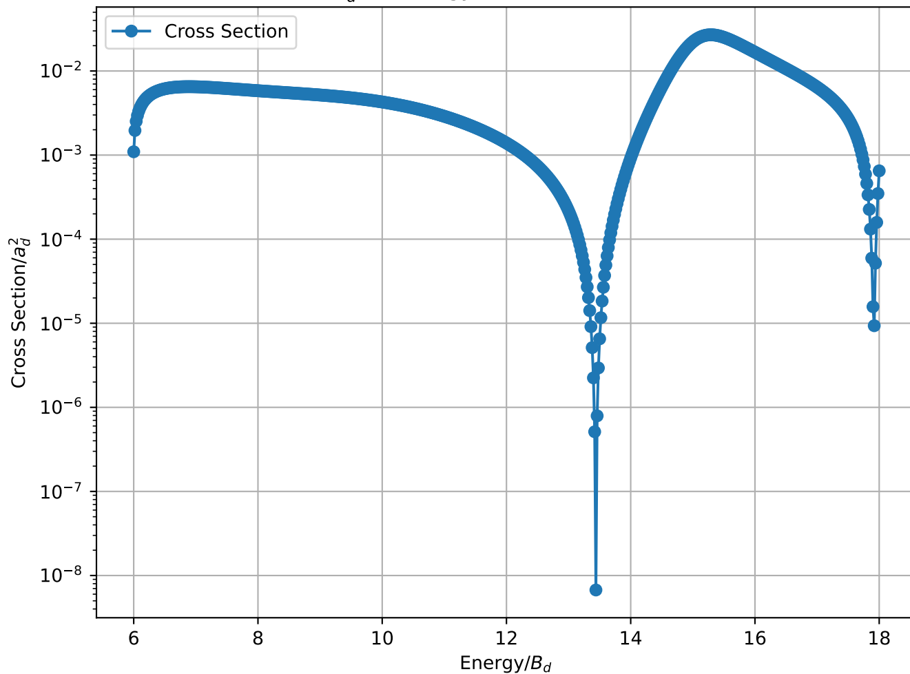
Cross Section/ a_d^2 vs Energy/ B_d for 1-2 B_3 = 4.00 MeV , L=10
