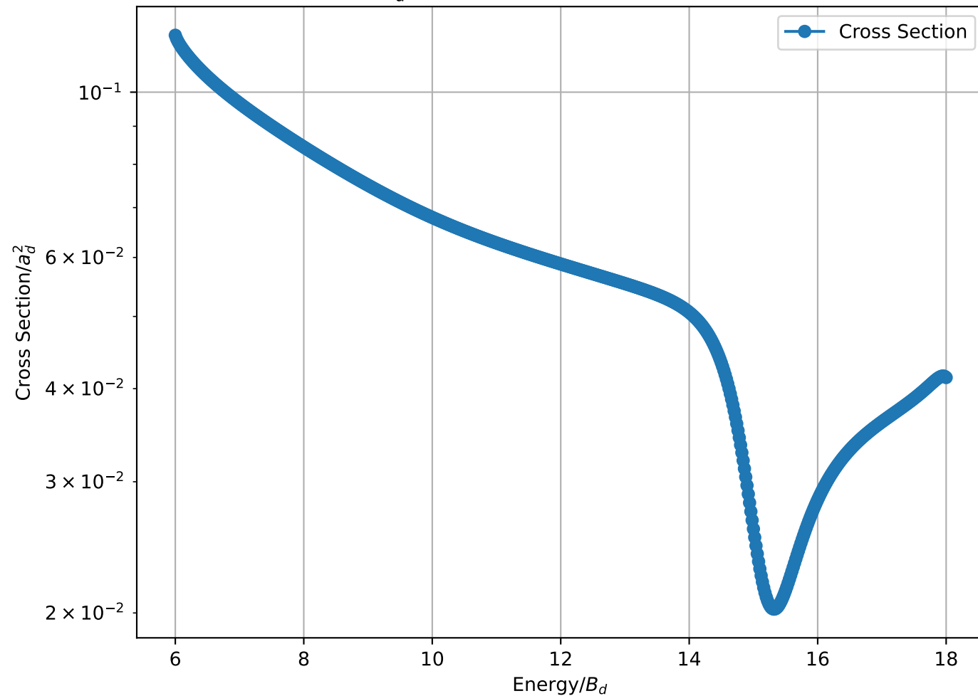
Cross Section/ a_d^2 vs Energy/ B_d for 2-2 B_3 = 4.00 MeV , L=10
