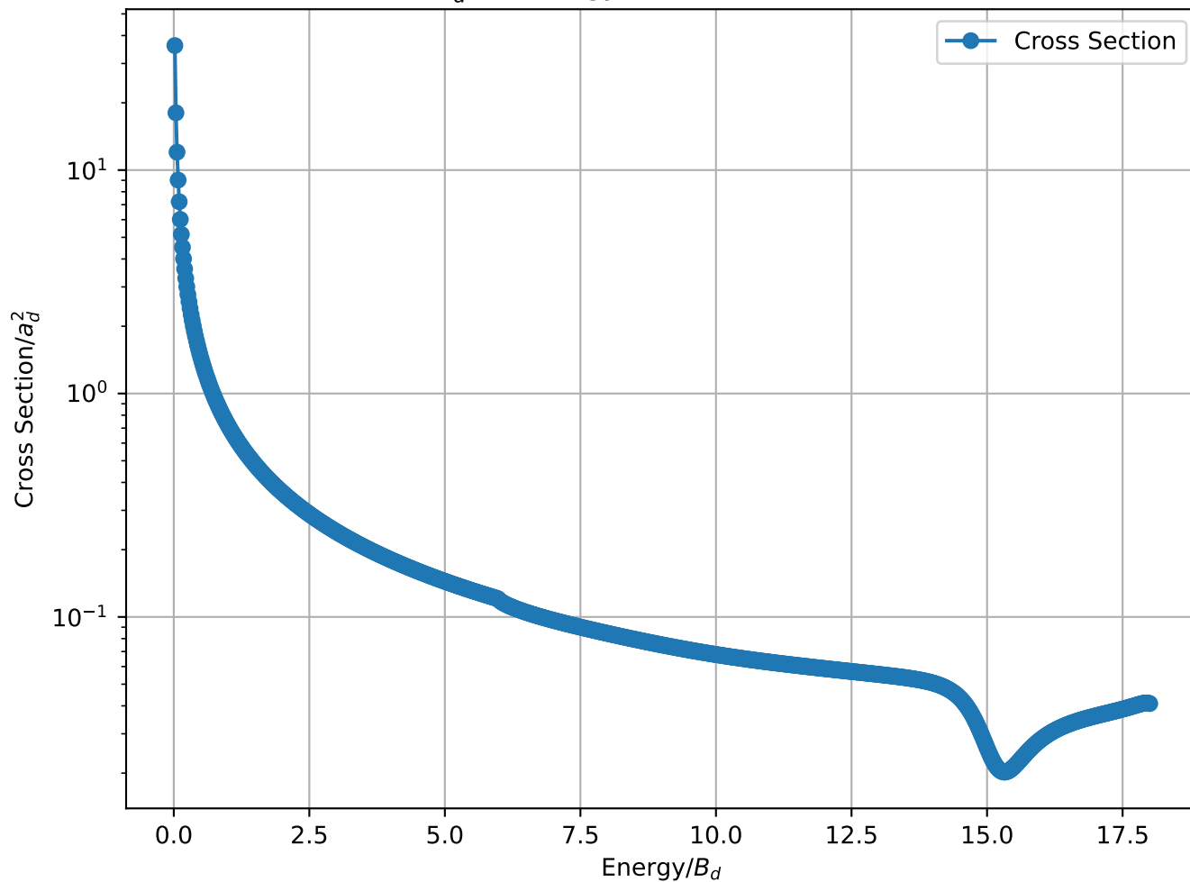
Cross Section/ a_d^2 vs Energy/ B_d for 1-1 B_3 = 4.00 MeV , L=10
