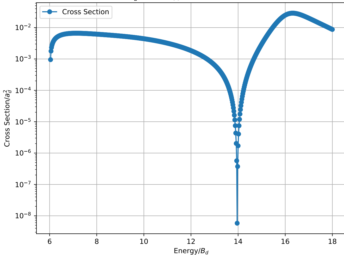
Cross Section/ a_d^2 vs Energy/ B_d for 1-2 B_3 = 4.00 MeV , L=6
