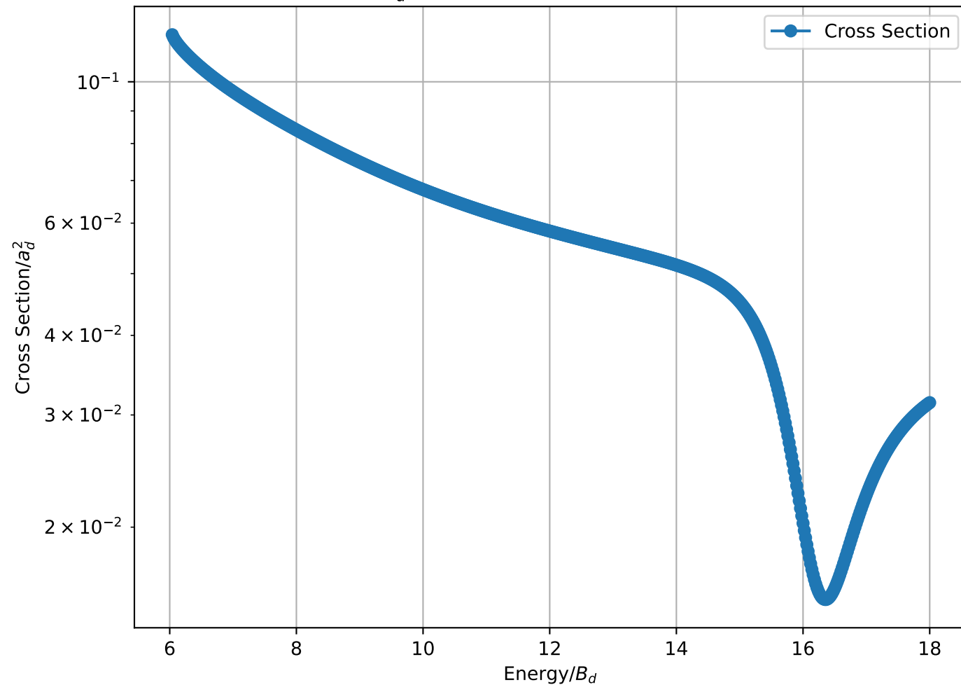
Cross Section/ a_d^2 vs Energy/ B_d for 2-2 B_3 = 4.00 MeV , L=6
