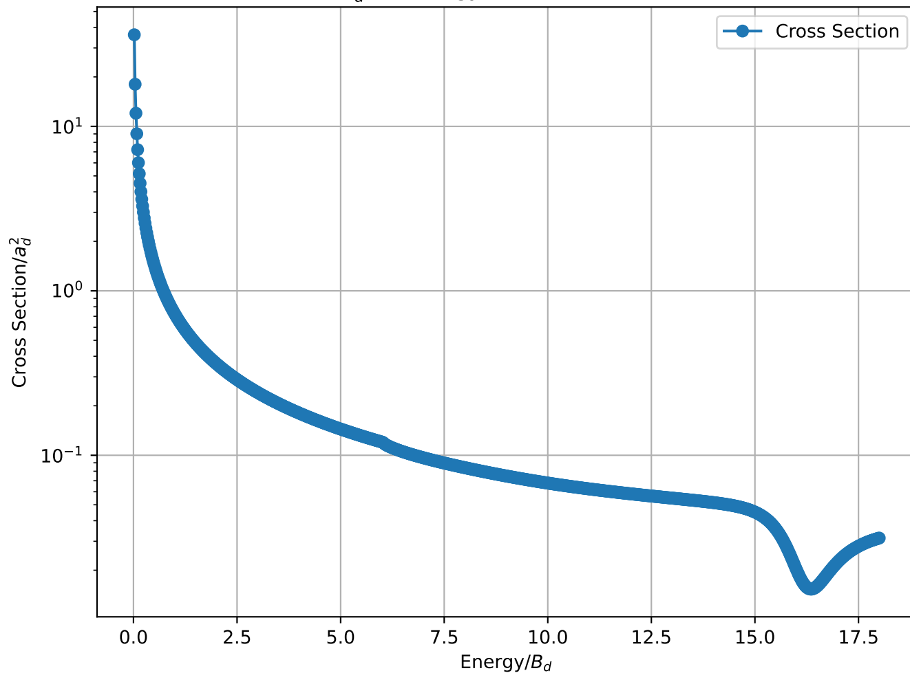
Cross Section/ a_d^2 vs Energy/ B_d for 1-1 B_3 = 4.00 MeV , L=6
