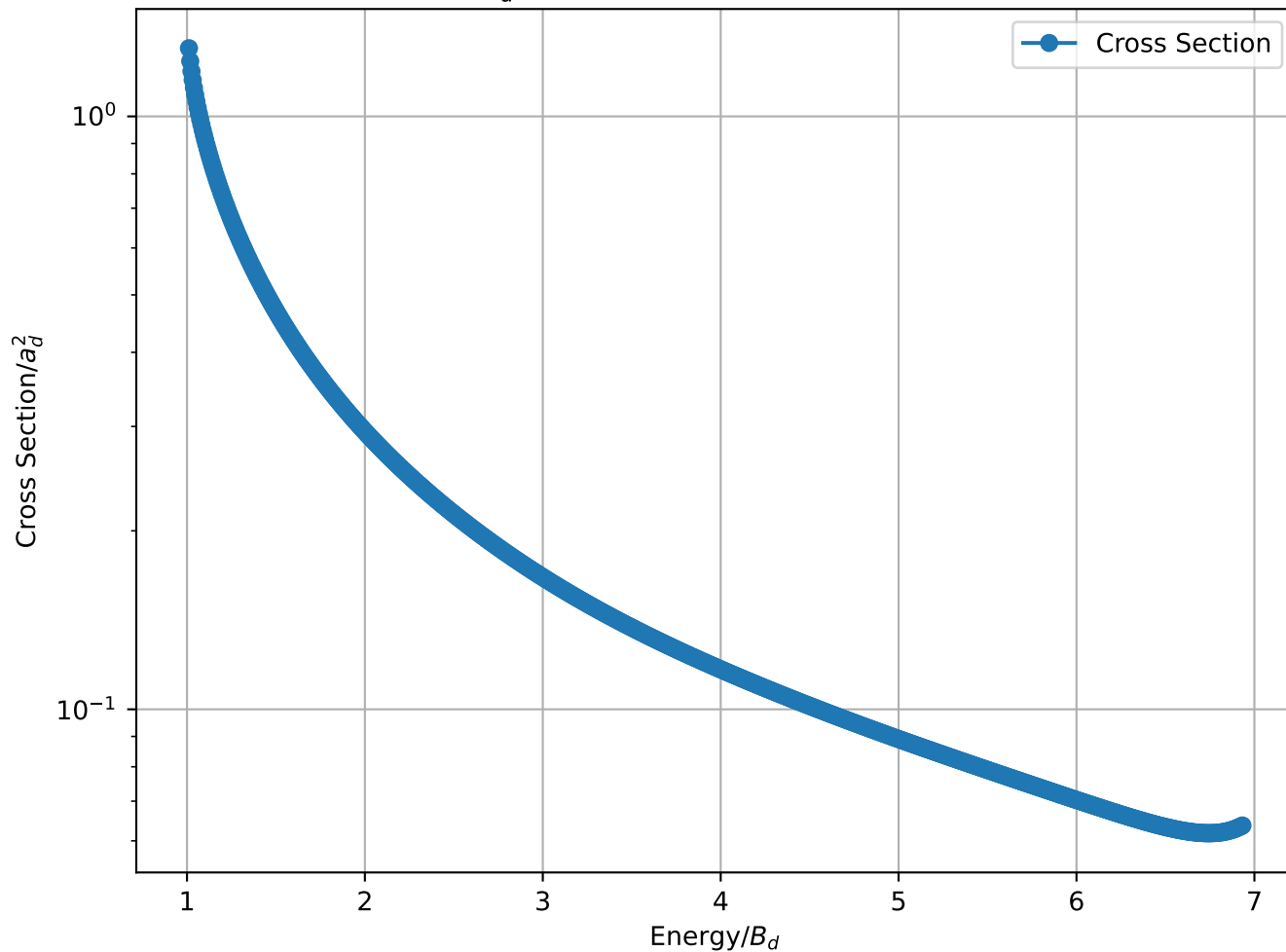
Cross Section/ a_d^2 vs Energy/ B_d for 2-2 B_3 = 3.00 MeV , L=6
