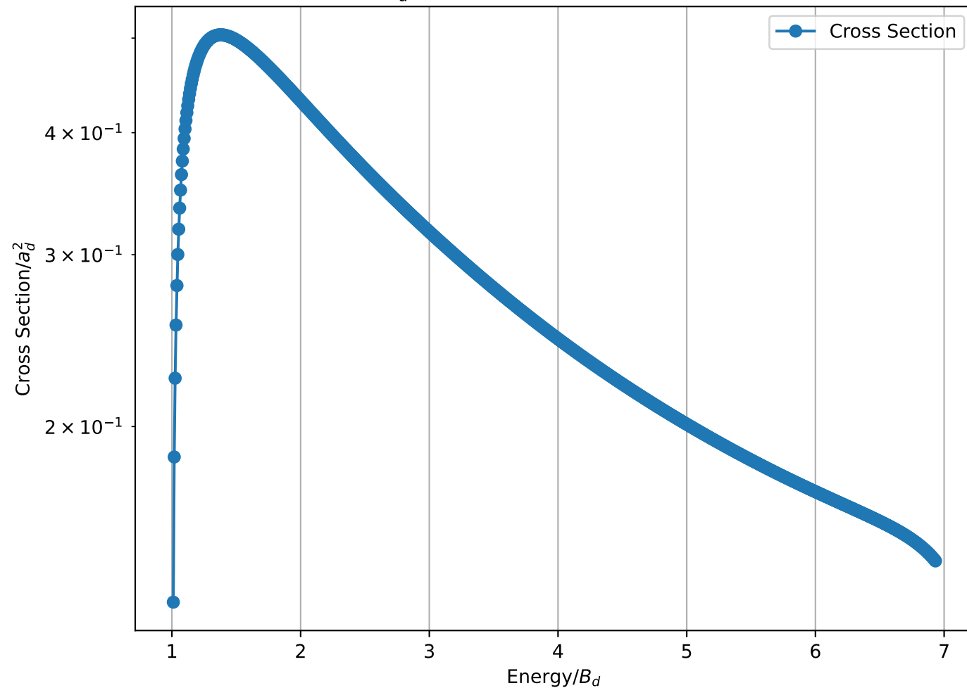
Cross Section/ a_d^2 vs Energy/ B_d for 1-2 B_3 = 3.00 MeV , L=6
