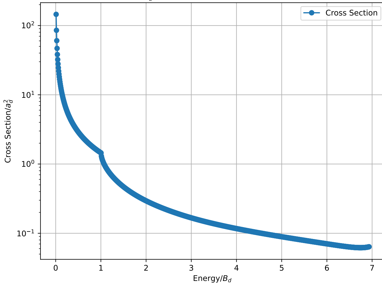
Cross Section/ a_d^2 vs Energy/ B_d for 1-1 B_3 = 3.00 MeV , L=6
