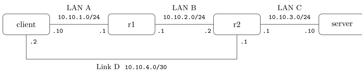
Figure 1: Network topology: four machines, LANs A–C and Link D.
