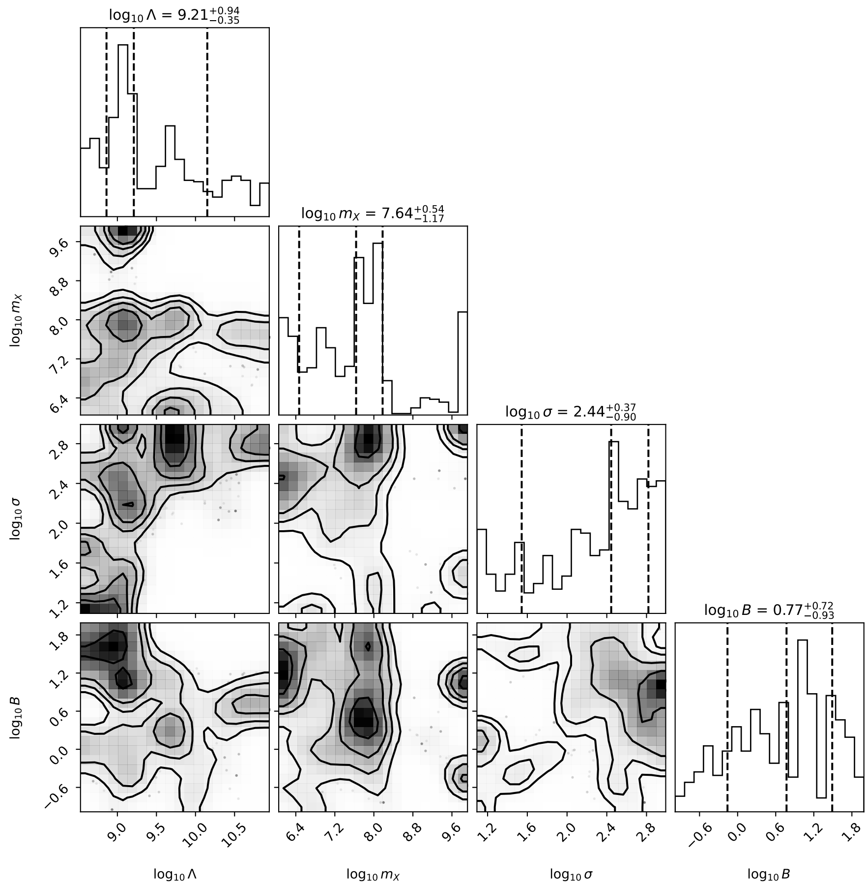
MCMC Parameter Scan — Convergence Diagnostics (Figure S1)
