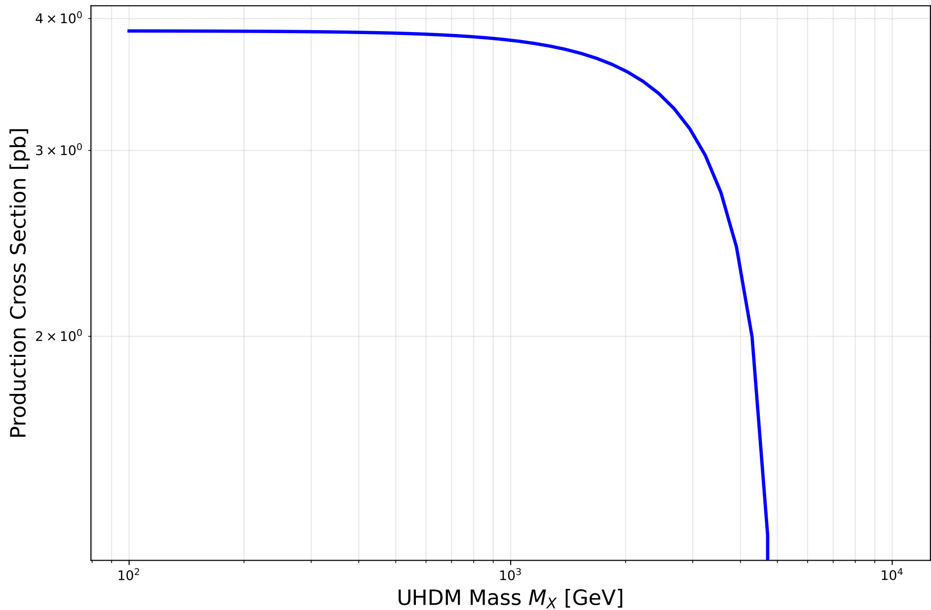
UHDM Production Rate vs Mass
