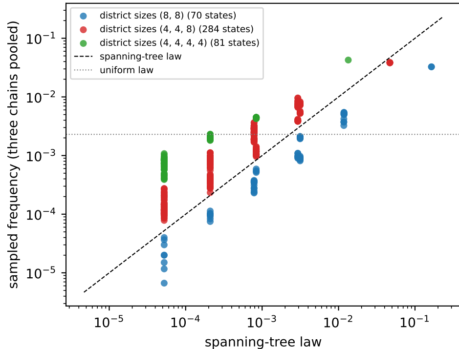
(a) all 435 feasible level-1 states, 4x4 grid
