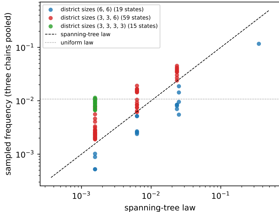
(a) all 93 feasible level-1 states
