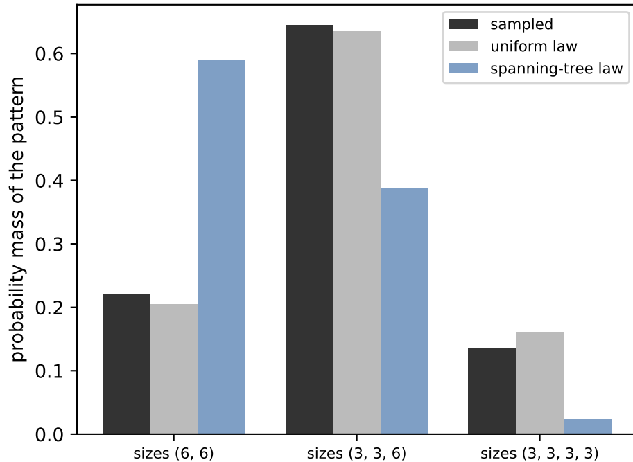
(b) mass by district-size pattern
