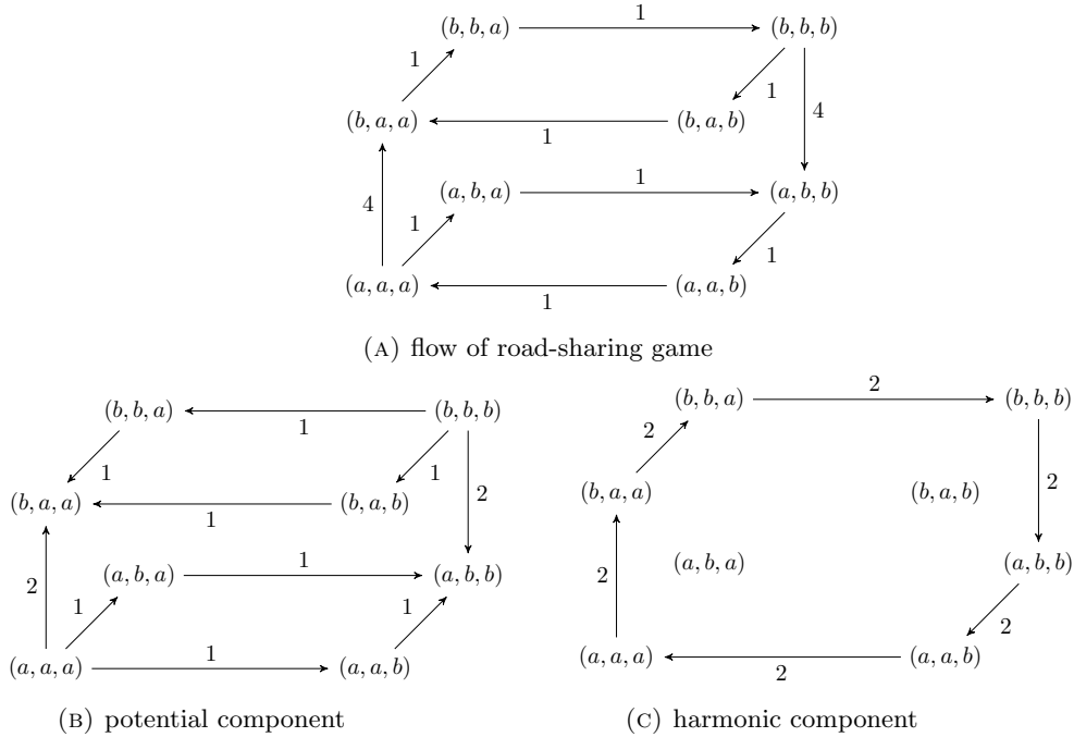
FIGURE 8. Helmholtz decomposition of the road sharing game. (Reproduced with slight modification from [15, Figure 1, p. 475])
