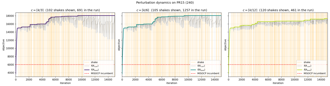
Figure 2: Perturbation dynamics on PR15 (240) for three cap divisors, the first 15 000 iterations of each run: current objective (grey), best-seen objective (colored), shake steps (orange) and the MISOCP incumbent (dashed).
