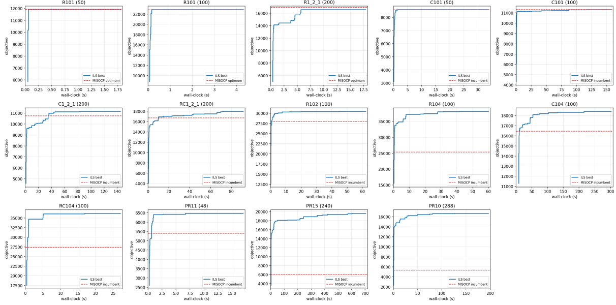
Figure 3: Best-seen objective against wall-clock time for replication 1 of Table 10, one panel per instance; each panel ends where its run ends. Dashed: the MISOCF value at the 3600 s cap.
