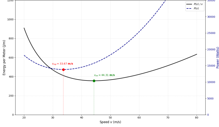
Figure 1: Maximum-range speed versus minimum-power speed.
