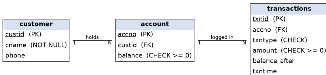
Fig. 12.1: ER diagram (customer 1:N account 1:N transactions).
