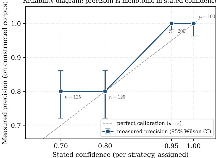
Reliability diagram: precision is monotonic in stated confidence
