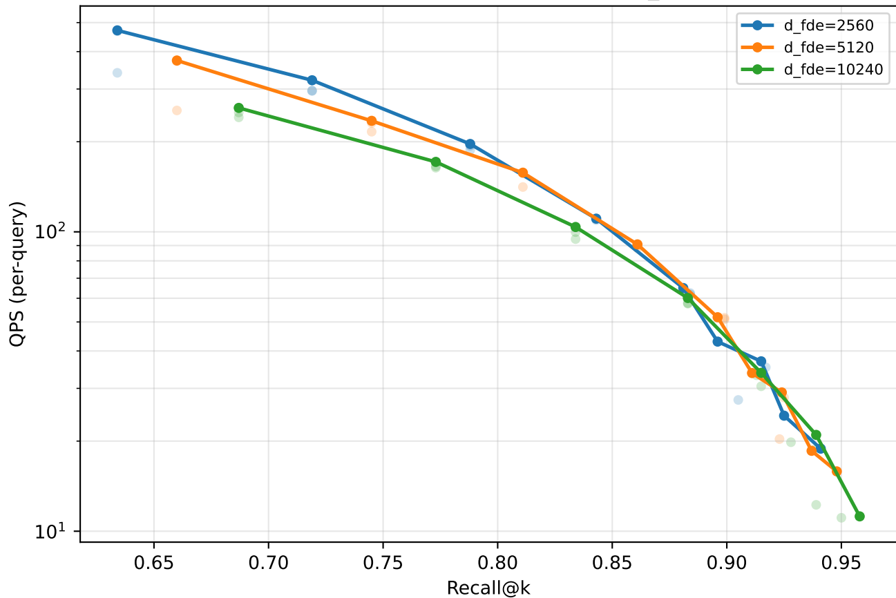
nq: MUVERA ablation (Pareto by d_fde)
