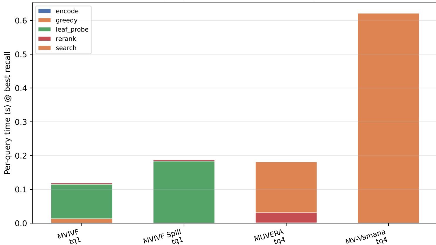
hotpotqa: timer breakdown [latency]
