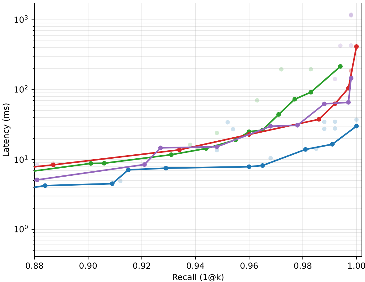
fiqa: recall vs latency (1000 / QPS_seq ms) [latency]
