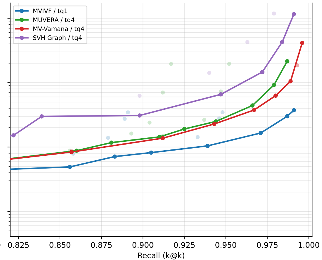
fiqa: recall vs latency (1000 / QPS_seq ms) [latency]
