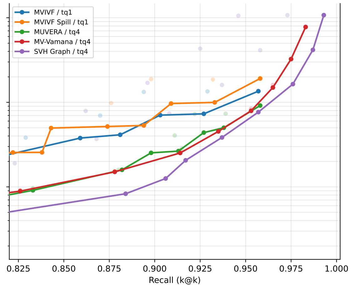
nq: recall vs latency (1000 / QPS_seq ms) [latency]
