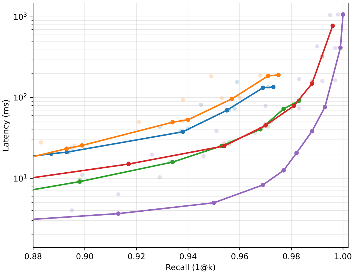
nq: recall vs latency (1000 / QPS_seq ms) [latency]
