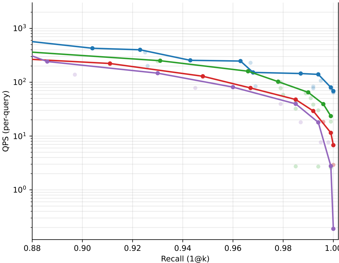
scidocs: recall vs QPS [latency]
