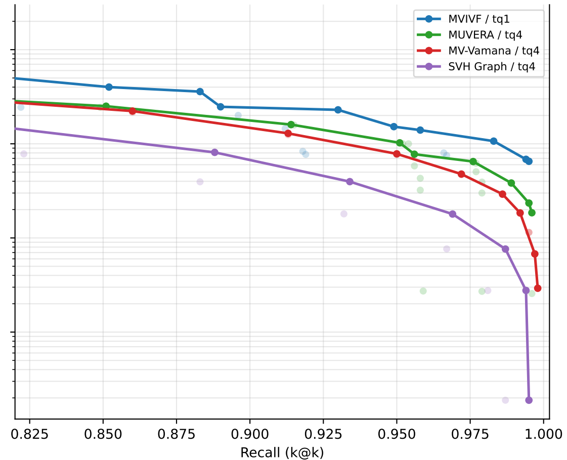
scidocs: recall vs QPS [latency]
