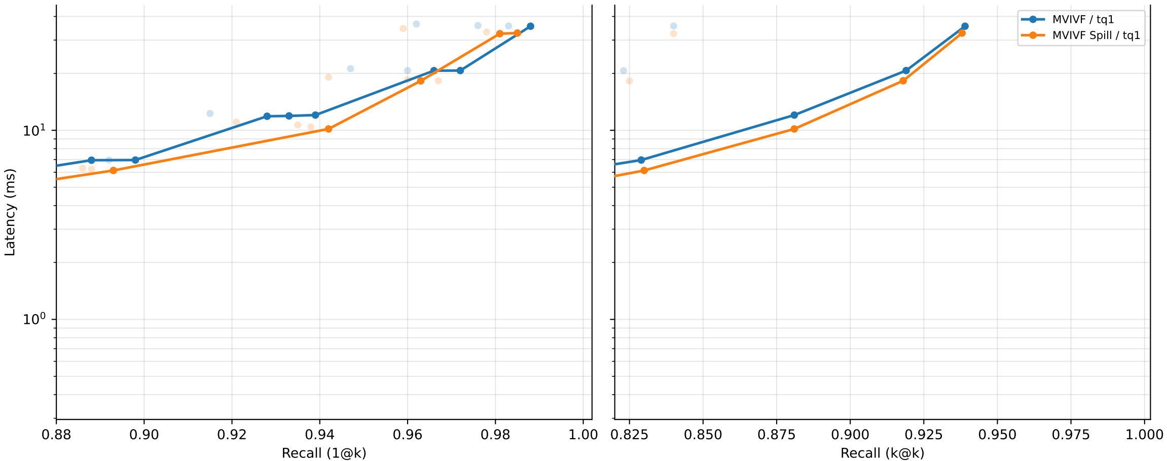
hotpotqa: recall vs latency (1000 / QPS_seq ms) [multi_latency]
