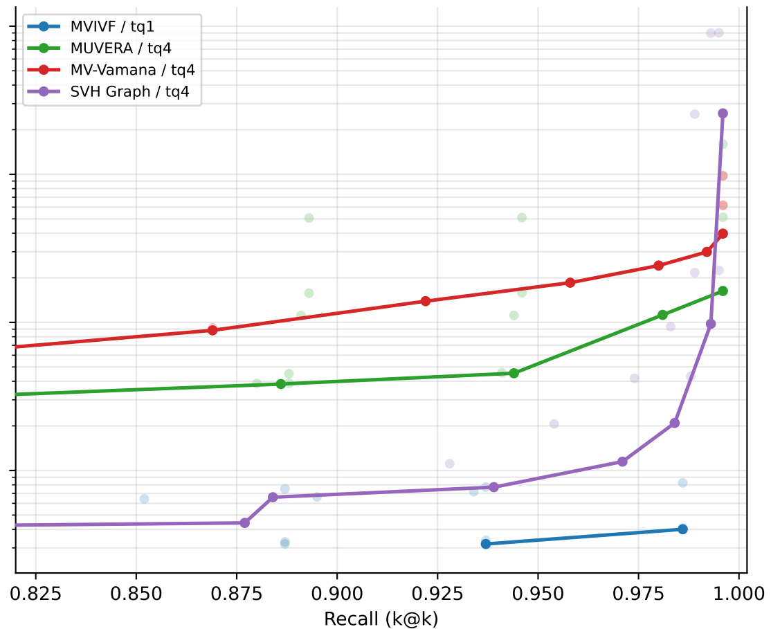
nfcorpus: recall vs latency (1000 / QPS_seq ms) [multi_latency]
