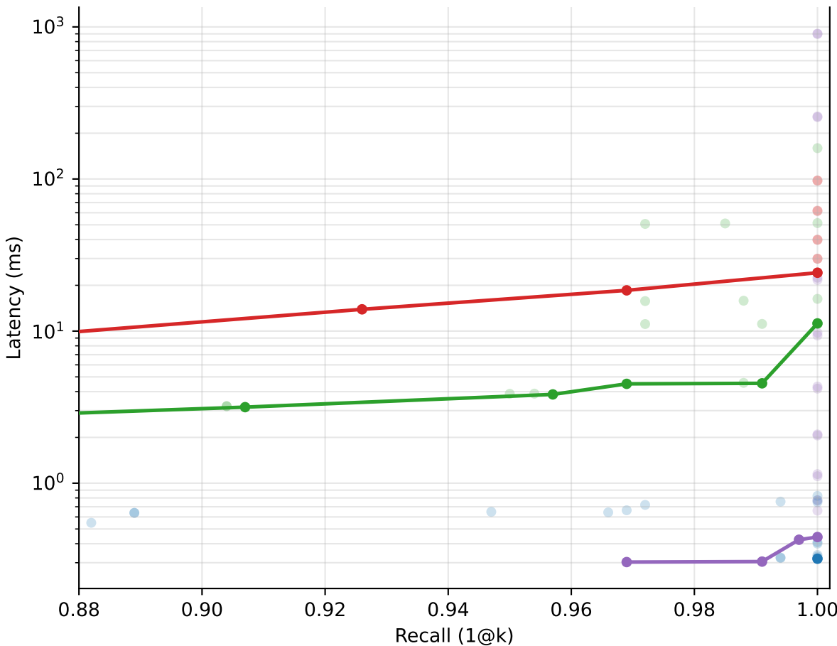
nfcorpus: recall vs latency (1000 / QPS_seq ms) [multi_latency]
