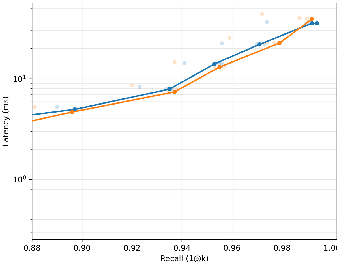
nq: recall vs latency (1000 / QPS_seq ms) [multi_latency]
