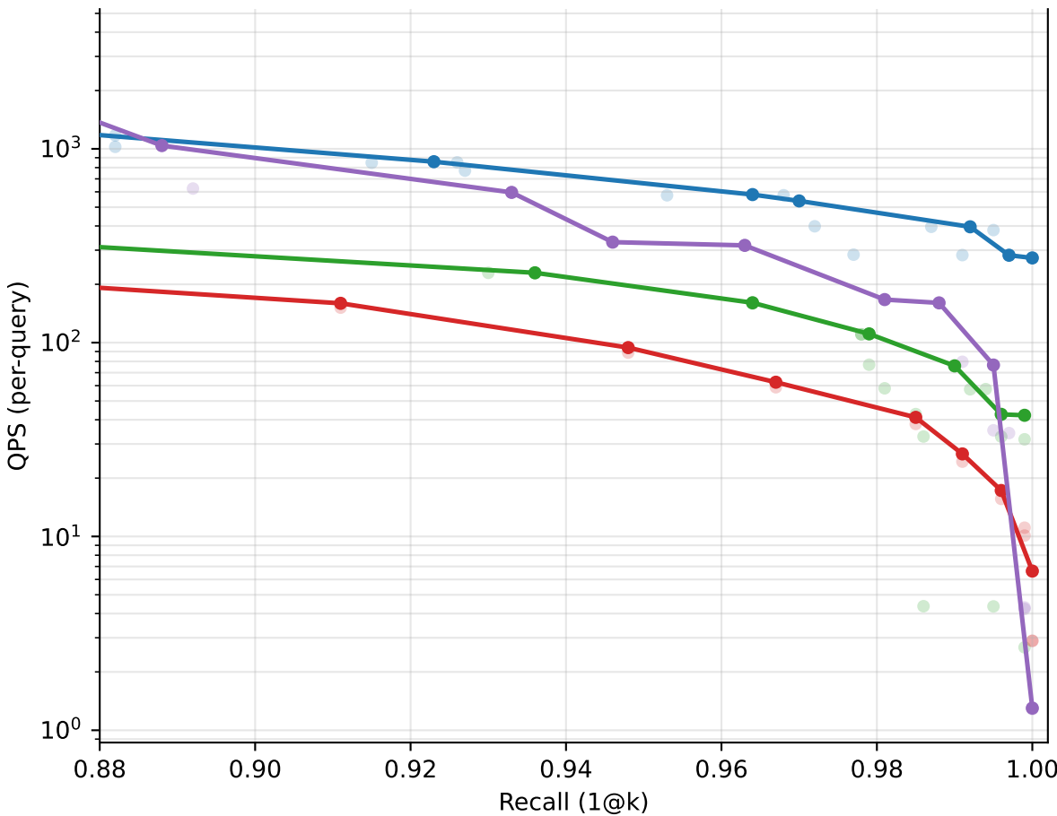
scidocs: recall vs QPS [multi_latency]
