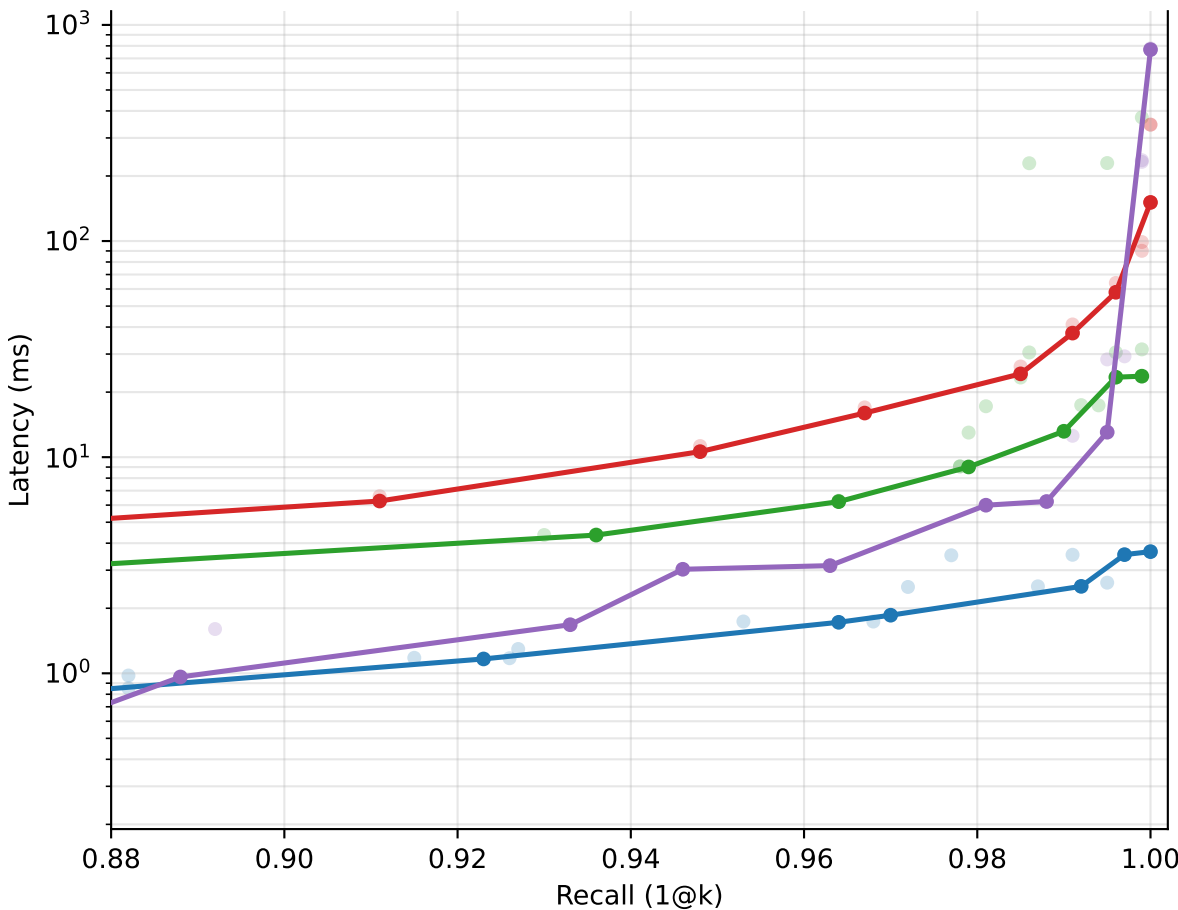
scidocs: recall vs latency (1000 / QPS_seq ms) [multi_latency]
