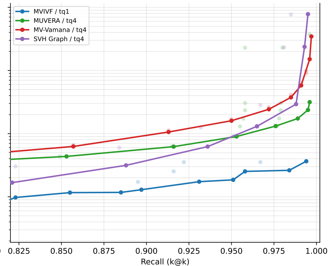
scidocs: recall vs latency (1000 / QPS_seq ms) [multi_latency]
